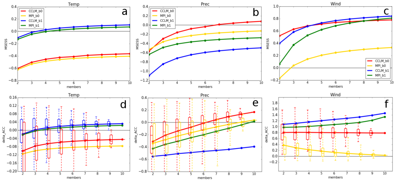
5 Figure 5: Skill scores for the multi-annual mean anomalies of lead years 1-5 of the CCLM_b0 (red), MPI_b0 (yellow), CCLM_b1 (blue), and MPI_b1 (green) ensembles depending on the ensemble size (x-axis, ranging from 2 to 10 members) over IP (cf. Fig. 1). MSESS for (a) temperature, (b) precipitation, and (c) wind speed; delta_ACC for (d) temperature, (e) precipitation, and (f) wind speed. In (d)-(f) box-whisker plots for the skill scores of all n-member combinations are shown to indicate the uncertainty due to the ensemble size. For MSESS and delta_ACC we have used the uninitialized historical ensemble as reference dataset. Note the different scaling of the y-axis. For details, please refer to main text.
