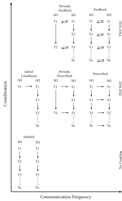
Fig. 2. Figure 2: Conceptual outline of the frequency of model communication and coordination of interaction between models from no coupling to one-way and two-way feedback.
