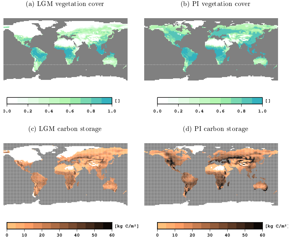
Figure 3. Vegetation cover and carbon storage in the LGM and PI ctrl simulations. Vegetation cover is given as fraction of grid cell covered with vegetation, and carbon storage in \text{kg C/m}^2 .
