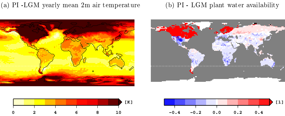
Figure 2. Differences between the LGM and PI climates obtained in the respective ctrl simulations: a) Difference in global mean near surface temperatures and b) difference in plant water availability. Here the values in the LGM state are subtracted from the values in the PI state. Land areas that are covered by ice in the LGM but not in the PI equilibrium state show soil humidity differences > 0.4 .
