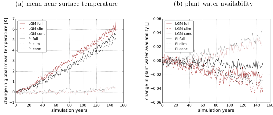
Figure 4. Climatic changes in the full simulation (continuous lines), clim simulation (dashed lines) and the conc simulation (dotted lines) due to rising \text{CO}_2 concentrations in the LGM experiment (red) and PI experiment (black). a) shows the globally averaged change in near surface temperature and b) in plant water availability.
