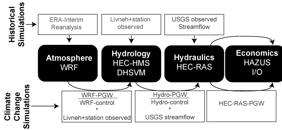
Figure 2. Diagram of the integrated modeling, including the models used and the input data for each model during the historical simulations (top) and the climate change simulations (bottom). Hydro-control represents both HEC-HMS and DHSVM-control simulations, while Hydro-PGW represents both HEC-HMS and DHSVM-PGW simulations.
