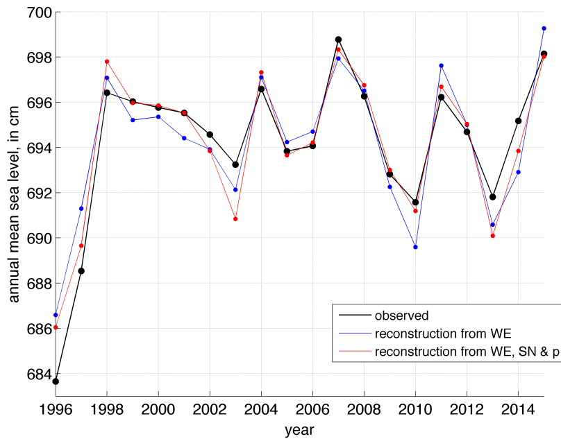
Figure 8. Observed annual mean sea level at Den Helder is replicated in black from Figure 2. The blue and red lines represent reconstructed annual mean sea levels based on atmospheric data. The blue line results from the annual mean west-east component of wind energy combined with the least squares fit of Figure 7. The red line uses a multiple regression involving both directions of the wind energy vector (i.e., west-east and south-north) as well as the annual mean atmospheric pressure at weather station Vlieland.
