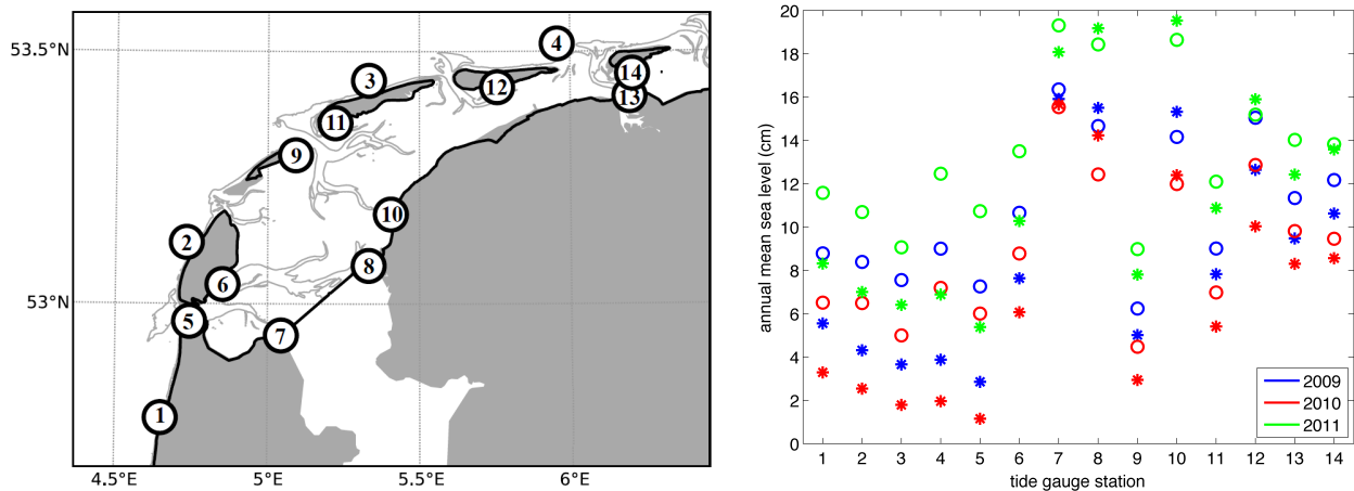
Figure 10. Annual mean sea level for the years 2009-2011: comparison between model results (asterisks) and observations (circles) for fourteen tide gauges in and around the Dutch Wadden Sea, whose positions are indicated in the map on the left.
