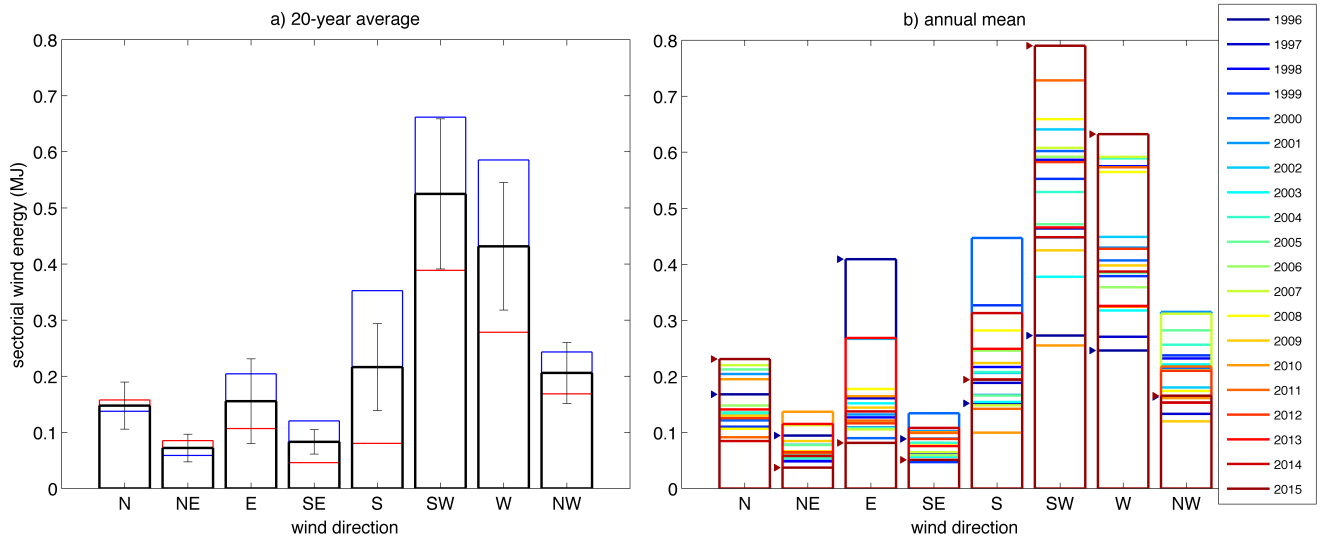
Figure 4. Annual mean wind energy at weather station Vlieland, divided in eight sectorial directions. In a) the average over the 20-year record (1996-2015), in black. The vertical line segments represent the standard deviations for each sector, as an indication of the typical inter-annual variability. Also shown are the averages of the summer half-year (in red) and winter half-year (in blue). In b) the sectorial annual mean wind energy for all individual years. For clarity, the extreme years 1996 (darkblue) and 2015 (darkred) are highlighted with triangles alongside the bars.
