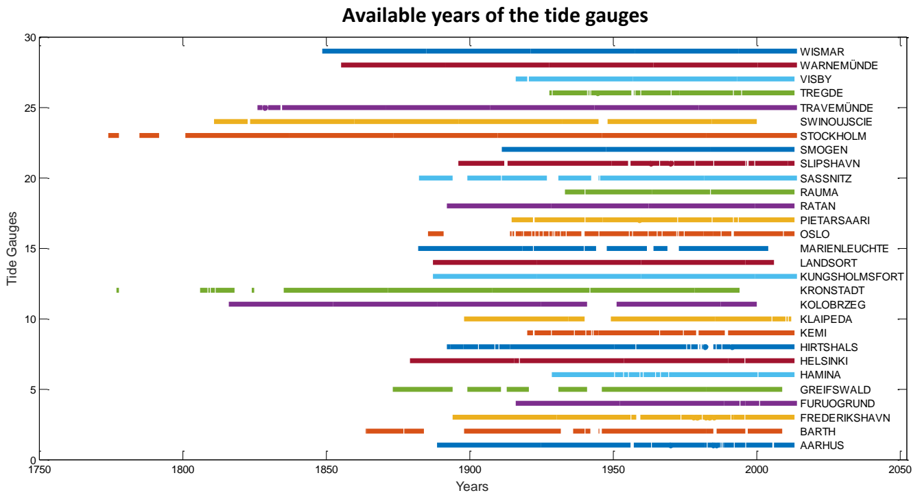
Figure 2: Time coverage of the tide gauge observations (monthly means). Numbers on the y-axis refer to the station number defined in Figure 1. Time series are coloured for better visibility.
