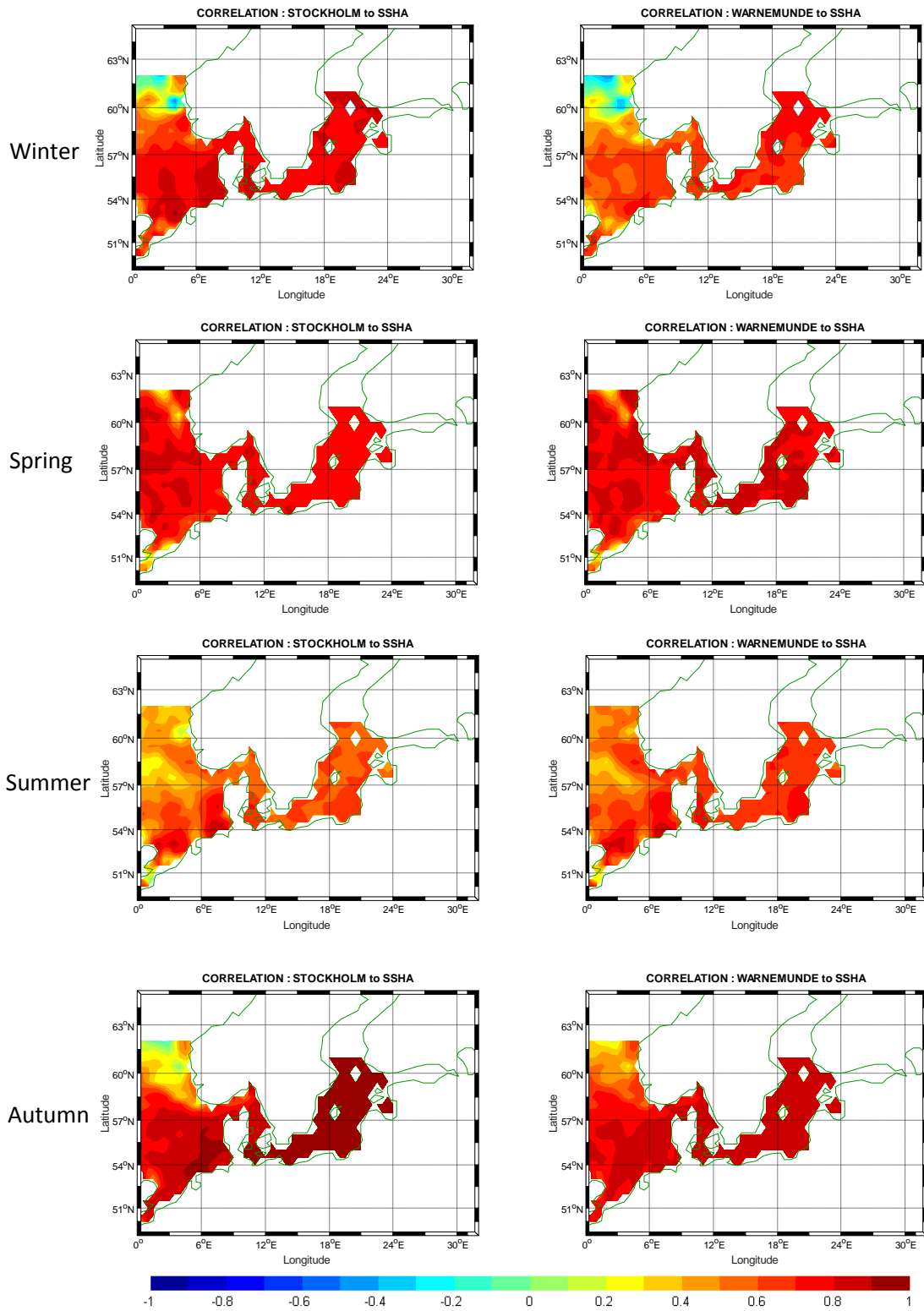
Figure 4: Correlations of decadal gliding trends between selected (Stockholm-left and Warnemünde-right) tide gauges and SSHA grids for all seasons shown in the order of winter-first row, spring-second row, summer-third row, autumn-last row (period: 1950-2008). The 95% significance level is \pm 0.25 for this record length.
