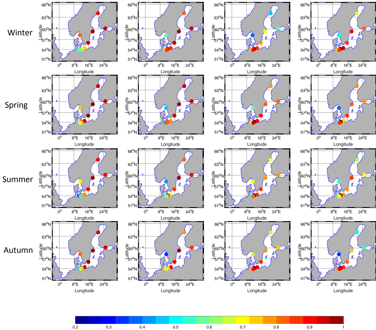
Figure 5: Correlation between sea-level at two representative tide gauges (Stockholm and Warnemünde) and at the rest of the tide gauges based on decadal trends. First (last) two columns present the correlation between Stockholm (Warnemünde) and the other tide gauges. For each tide gauge, the left (right) column shows the correlations obtained with the observed (residual) record. The maps are ordered in the line of winter-first row, spring-second row, summer-third row, autumn-last row. The 95% significance level is \pm 0.19 at the 95% for this record length. Note that correlation scale ranges from 0.2 to 1.
