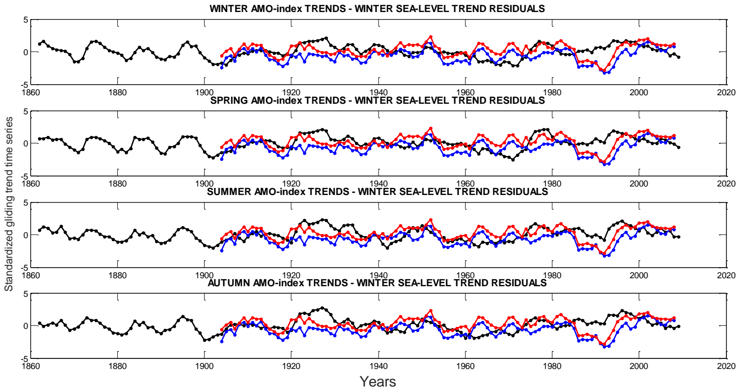
Figure 10: The standardized (unitless) decadal gliding trend time series of the AMO-index (black) and tide gauge residuals (blue-Stockholm, red-Warnemünde).
