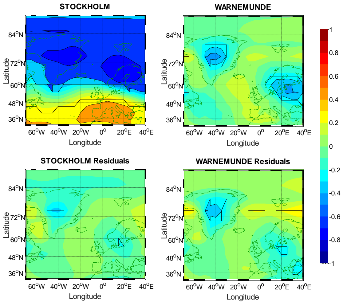
Figure 6: The correlation patterns between SLP fields and Stockholm and Warnemünde before (top) and after (bottom) removing the atmospheric signal in wintertime. The areas indicating significant correlations are delineated with contour lines. The 95% significance level is \pm 0.19 for this record length.
