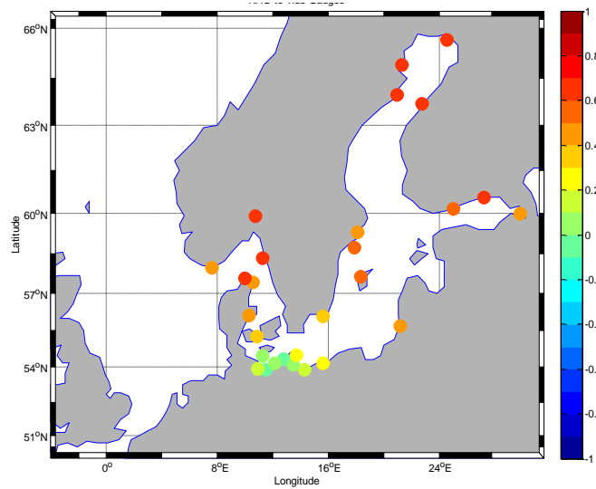
Figure 3: Correlations of decadal gliding trends between the NAO-index and 29 tide gauges for wintertime (1900-2012). The 95% significance level is \pm 0.19 for this record length.
