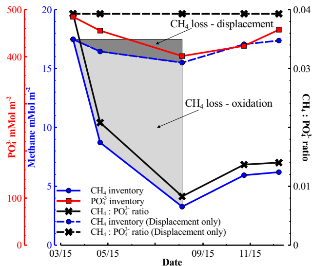
Figure 3. Evolution of the inventories of \text{CH}_4 (solid blue line with dots) and \text{PO}_4^{3-} (solid red line with squares) below 70 m at BY15, and the molar inventory ratio \text{CH}_4:\text{PO}_4^{3-} over the year 2015 (solid black line with crosses). Results from all measured depths at all sampling times were included in the integration, with the exception data from June, which was omitted due to the loss of deep water \text{CH}_4 samples. Pictured also is the hypothetical evolution of the \text{CH}_4 inventory (dashed blue line with dots) if the \text{CH}_4:\text{PO}_4^{3-} ratio (dashed black line with crosses) had remained constant during the year, i.e. the effect of water mass displacement was equal for \text{CH}_4 and \text{PO}_4^{3-} . The lighter grey area represents the estimated loss of \text{CH}_4 due to oxidation and the darker grey represents the loss due to displacement. Note the different scales of the y-axes.
