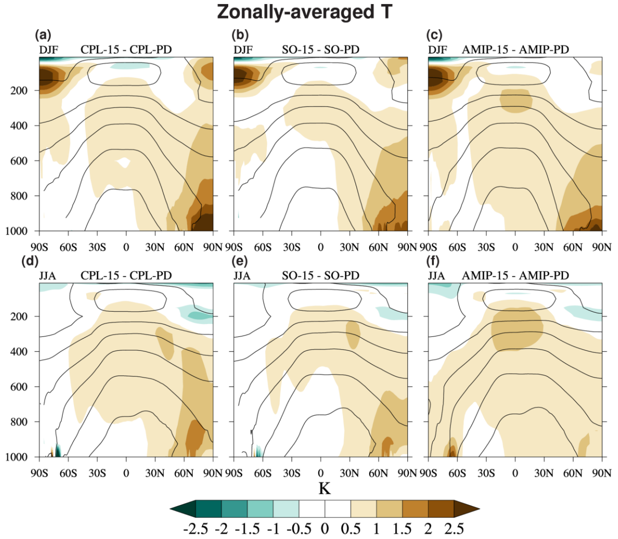
Figure 9: zonal-mean temperature response (K) relative to PD (colors) and climatology (solid black contours; 210 K to 285 K in increments of 15 K) for the 1.5 K experiment from NorESM1-Happi (left; a, d), NorESM1-HappiSO (middle; b, e), and NorESM1-HappiAMIP (right; c, f). Fields are shown for DJF (top row; a–c) and JJA (bottom row; d–f). The fields are shown for the default periods given in Sect. 3. Units are K (a–f).
