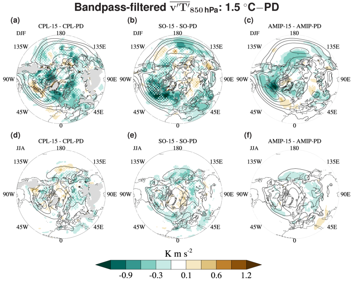
Figure 15: changes in the low-level storm-track activity relative to PD (colors) and PD climatology (black contours; -12 to 12 \text{K m s}^{-2} in increments of 4 \text{K m s}^{-2} ) for the 1.5 K experiment from NorESM1-Happi (left; panels a and d), NorESM1-HappiSO (middle; panels b and e) and NorESM1-HappiAMIP (right; panels c and f) for DJF (top; panels a–c) and JJA (bottom; panels d–f). The storm tracks are represented in terms of the bandpass-filtered eddy heat flux \overline{v'T'} at 850 hPa. The white dots indicate that the differences are not significant at the 5 % level according to the Welch t-test. The fields are shown for the default periods given in Sect. 3. Units are \text{K m s}^{-2} (a–f).
