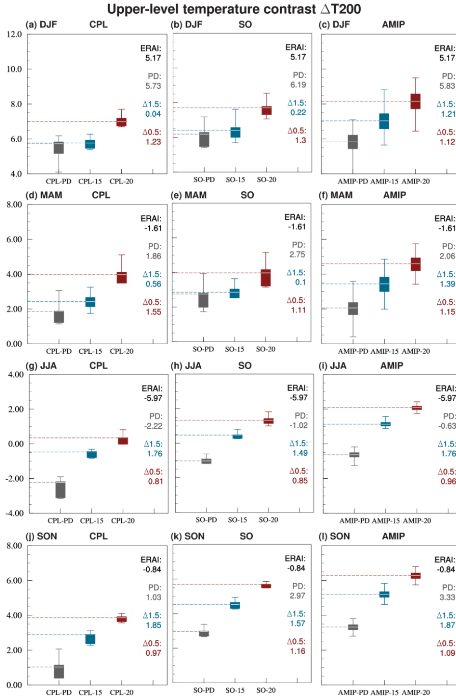
Figure 10: upper tropospheric temperature contrast in the PD (grey), 1.5 K (blue), and 2.0 K (red) experiments from NorESM1-Happi (left column; a,d,g,j), NorESM1-HappiSO (middle column; b,e,h,k), and NorESM1-HappiAMIP (right column; c,f,i,l) for DJF (top row; a–c), MAM (middle row; d–f), JJA (third row; g–i), and SON (bottom row; j–l). The upper-level temperature contrast \Delta T_{200} is defined as the 200 hPa temperature difference between an area over the tropics (30 °S–30 °N) and an area over the Arctic (poleward of 60 °N). The white lines within the boxes indicate the median values, the boxes indicate the inter-quartile range, and the whiskers the full spread of the different decades in each experiment (9 in NorESM1-Happi, 9 in NorESM1-HappiSO, and 125 in NorESM1-HappiAMIP). The dashed horizontal lines emphasize the median values, numbers are shown on the right side of each panel for ERA-Interim (top black), PD (second
