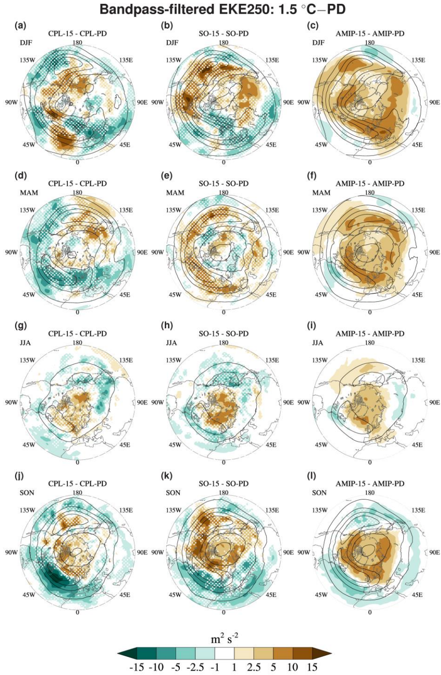
Figure 13: changes in upper-level storm-track activity relative to PD (colors) and climatology (black contours; 40 to 240 \text{m}^2 \text{s}^{-2} in increments of 40 \text{m}^2 \text{s}^{-2} ) for the 1.5 K experiment from NorESM1-Happi (left; a, d, g, j), NorESM1-HappiSO (middle column; b, e, h, k), and NorESM1-HappiAMIP (right; e, f, i, l) for DJF (top row; a–c), MAM (middle row; d–f), JJA (third row; g–i), and SON (bottom; j–l). The storm tracks are represented in terms of bandpass-filtered EKE (eddy kinetic energy) at 250 hPa. The white dots indicate that the differences are not significant at the 5 % level according to the Welch t-test. The fields are shown for the default periods given in Sect. 3. Units are \text{m}^2 \text{s}^{-2} (a–l).
