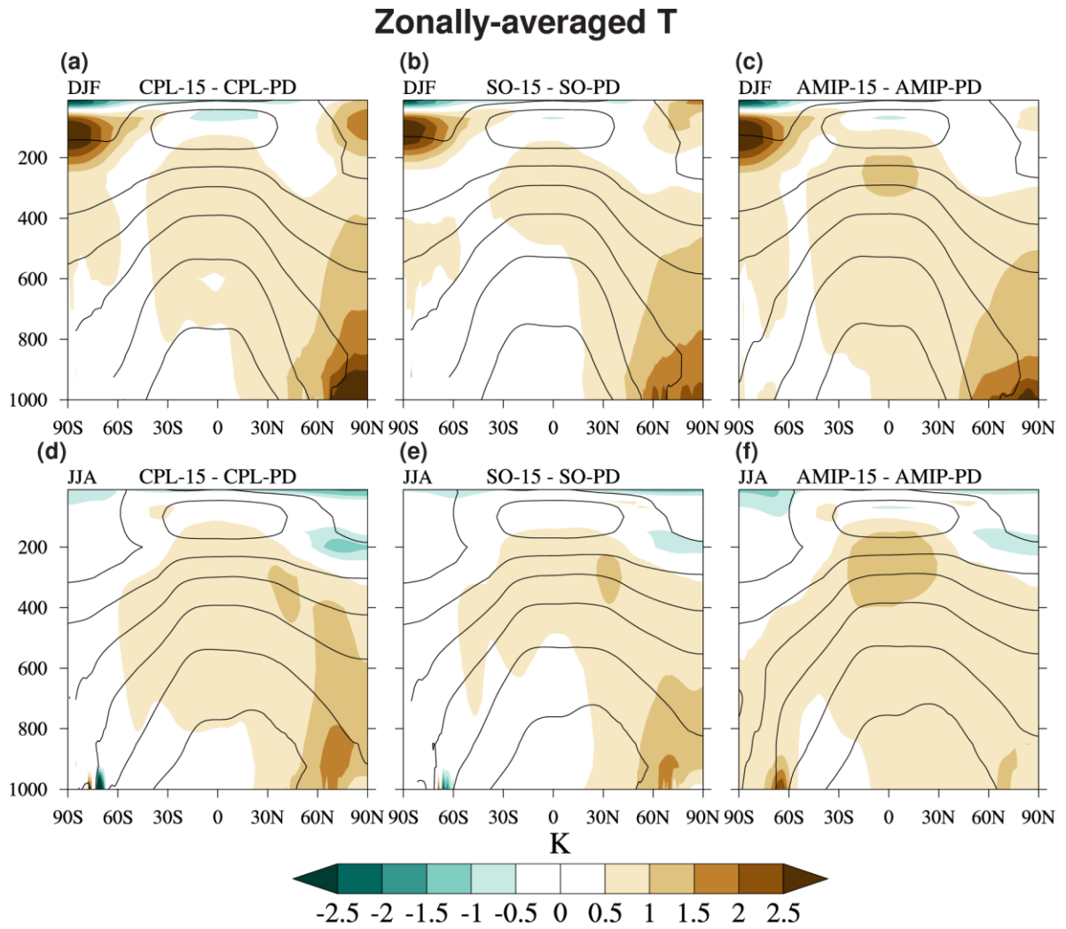
Figure 9: zonal-mean temperature response ( K ) relative to PD (colors) and climatology (solid black contours; 210 K to 285 K in increments of 15 K) for the 1.5 K experiment from NorESM1-Happi (left; a, d), NorESM1-HappiSO (middle; b, e), and NorESM1-HappiAMIP (right; c, f). Fields are shown for DJF (top row; a–c) and JJA (bottom row; d–f). The fields are shown for the default periods given in Sect. 3. Units are K (a–f).
