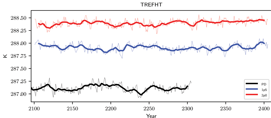
Fig. 1. The evolution of global mean temperature in the SO simulations for present day 2006-2015 (PD, black), the 1.5 (1p5, blue), and the 2.0 (2p0, red) degrees warmer world than pre-industrial. The number in
