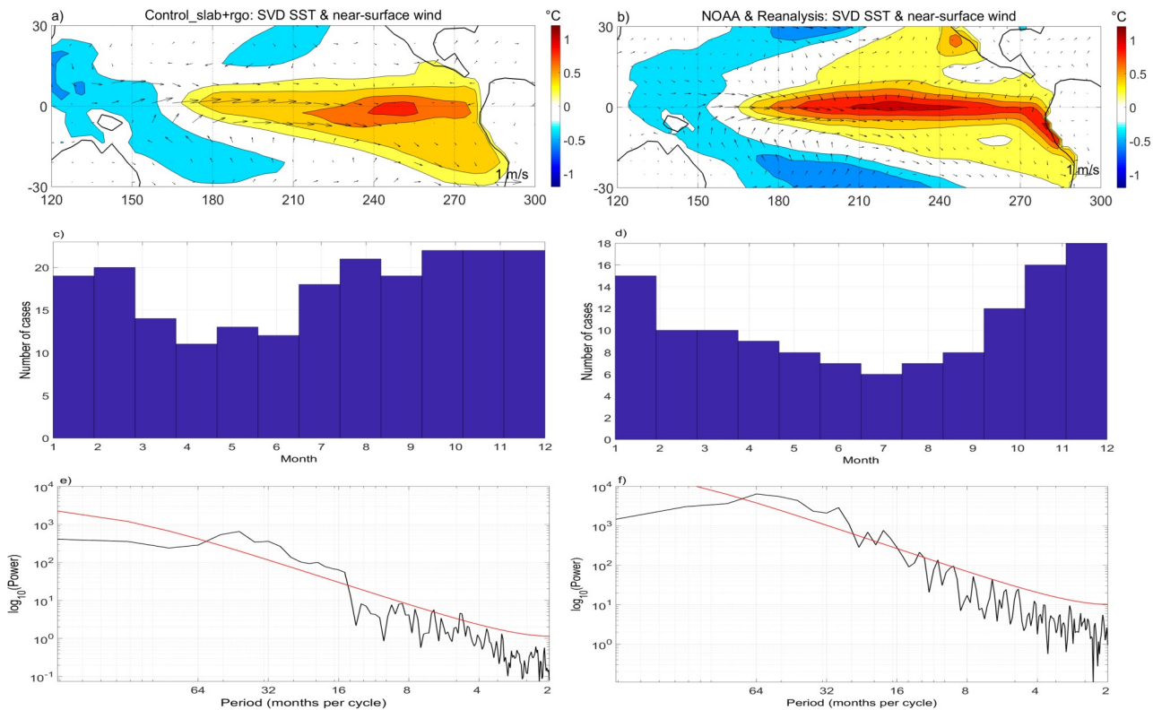
Figure 2: First SVD pattern of SST and near-surface winds in the tropical Pacific Ocean (30°S-30°N, 120°E-300°E) for the Control_slab+rgo experiment (left) and NOAA SST and reanalysis data (right; Smith et al., 2008; Kalnay et al., 2006). a. and b.: Spatial pattern; contour interval 0.2°C. c. and d.: Histogram showing phase- locking to the seasonal cycle. e. and f.: Spectral analysis, the red line indicates the red noise spectrum.
