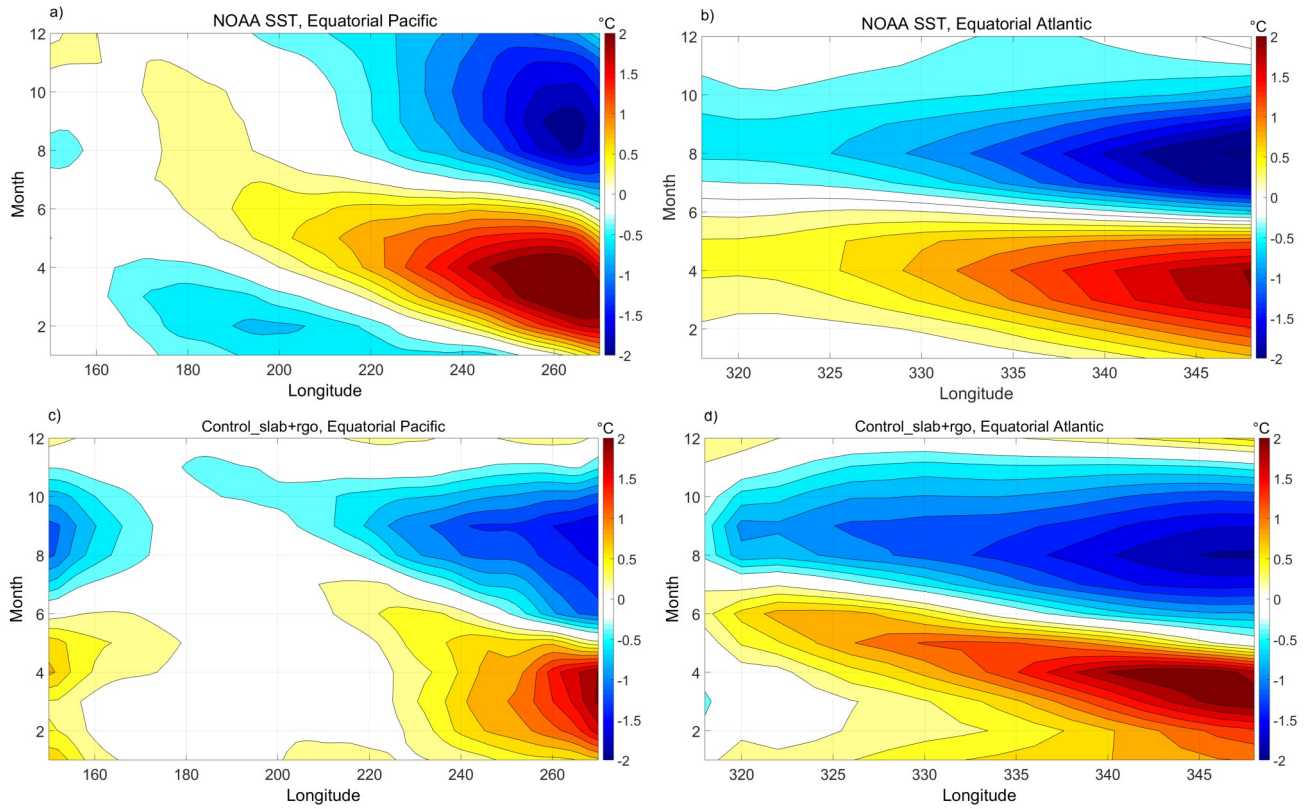
Figure 1: a. and b.: De-meaned SST seasonal cycle from NOAA SST data (Smith et al., 2008) in the Equatorial Pacific (2°S- 2°N, 150°E-270°E) and Atlantic (2°S-2°N, 320°E-345°E), respectively. c. and d.: De-meaned SST seasonal cycle for Control_slab+rgo in the Equatorial Pacific and Atlantic, respectively. Contour interval: 0.2°C.
