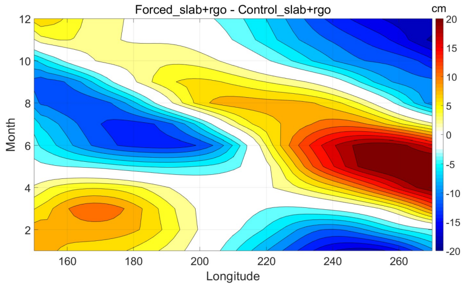
Figure 11: Equatorial Pacific Ocean (2°S-2°N, 150°E-270°E) de-meaned thermocline depth anomalies seasonal cycle for the : a. Forced_slab and b. Forced_slab+rgo experiments, respectively . Contour interval: 2 cm
