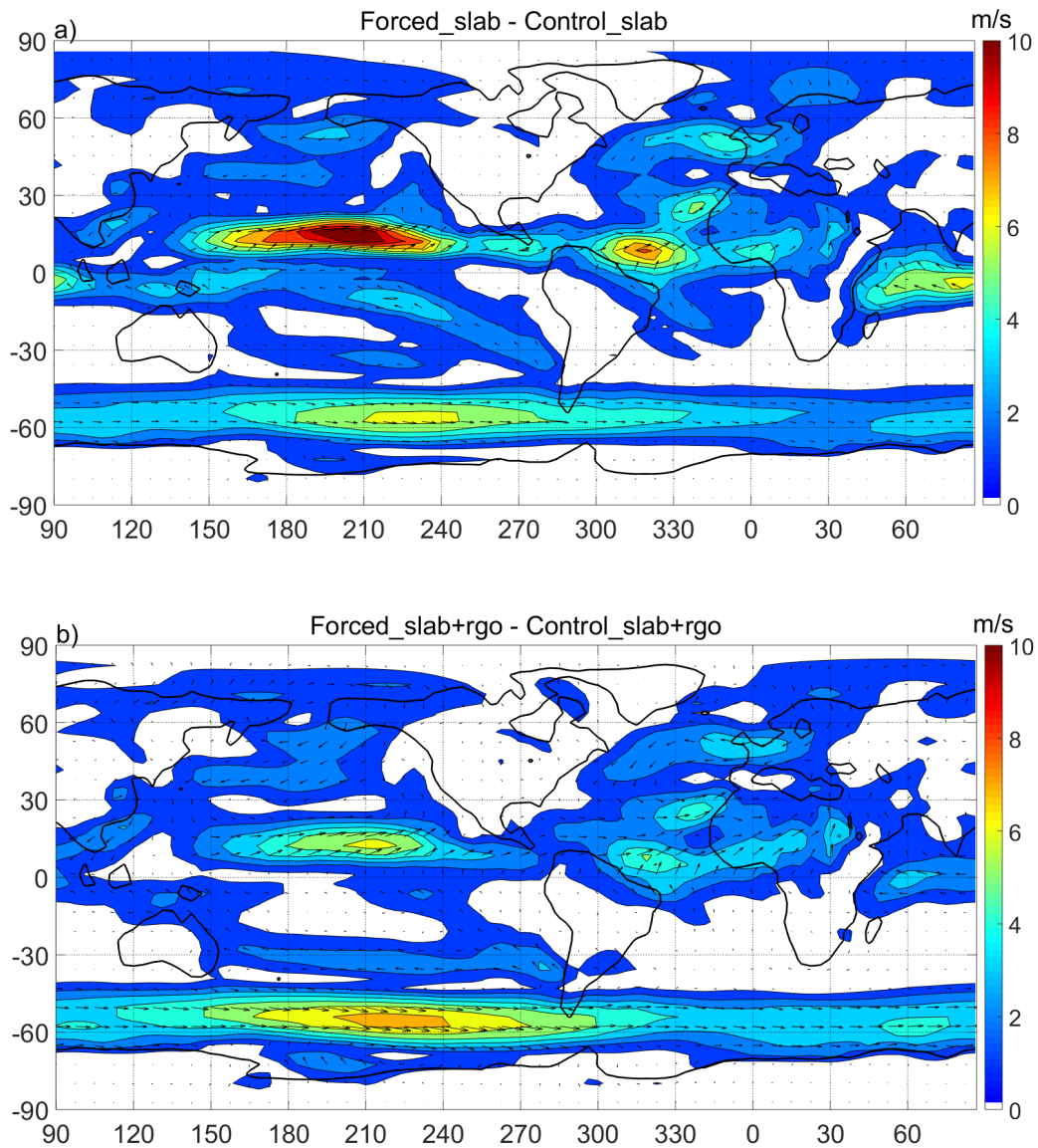
Figure 6: Annual mean anomalies with respect to the control of near-surface (950 hPa) wind for: a. Forced_slab and b. Forced_slab+rgo , respectively. Contour interval 1 m/s.
