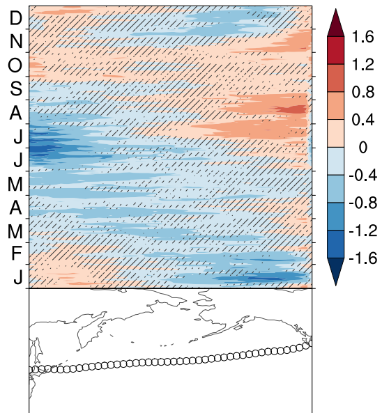
Figure 7. Multi-model mean shift of the North Pacific eddy-driven jet (shading, in degrees latitude) in the 2.0°C experiment compared to the PD experiment as a function of longitude and time. Hatching masks out regions where there is no model consensus (fewer than four out of five models agree) on the sign of the response. The bottom panel shows the climatological position of the jet in the PD experiment. Jet latitude is calculated following Simpson et al. (2014).
