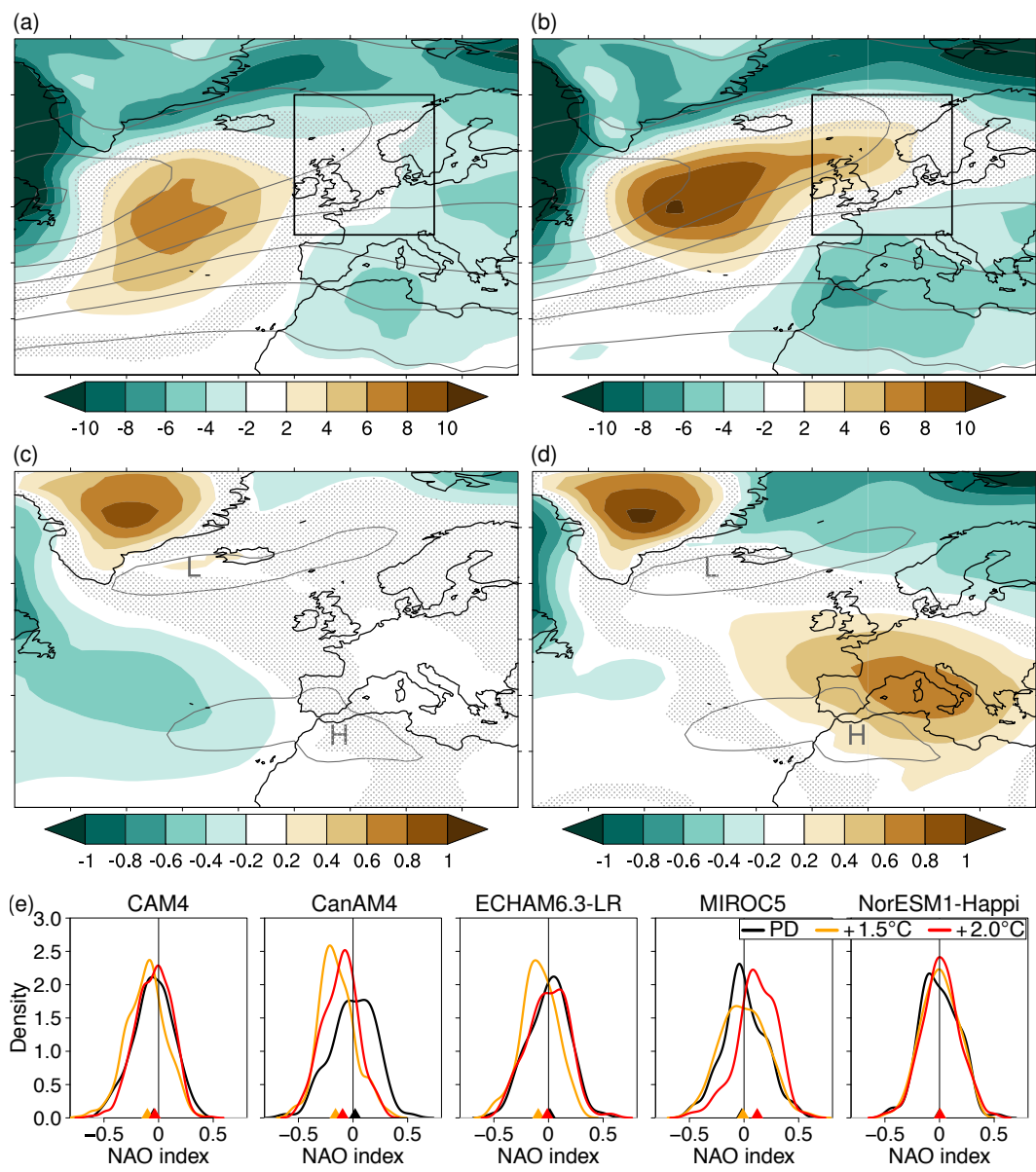
Figure 15. Multi-model mean response of winter (DJF) MSLP storm track and sea level pressure over the Euro-Atlantic sector in (a,c) 1.5°C and (b,d) 2.0°C relative to PD (shading, units: hPa) along with the PD climatology (contour interval 5 hPa in a,b; 1000 and 1025 hPa contours in c,d). Stippling in maps masks out regions where the response is very weak (signal-to-noise ratio |\beta/\sigma| < 0.1 ). (e) Distributions of the NAO index showing the spread and median (triangle) for each model and experiment.
