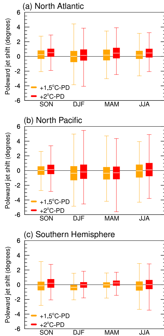
Figure 6. Multi-model mean shift of the eddy-driven jet in the 1.5°C (orange) and 2.0°C (red) experiments relative to the PD experiment for each season in the North Atlantic sector (60°W–0), North Pacific sector (135°E–235°E) and Southern Hemisphere. The white horizontal line in the boxes indicates the median, the boxes indicate the interquartile range, and the whiskers indicate the spread across all ensemble members for all models. Jet latitude is determined according to the method of Woollings et al. (2010). The mean shifts are very close to, but different from, zero based on 95% confidence intervals from 10,000 bootstrapped realizations of the full HAPPI ensemble (926 members over all models), with the exception of the following seasons/sectors: for 1.5°C–PD, North Atlantic DJF, North Pacific JJA/SON, Southern Hemisphere MAM; for 2.0°C–PD, North Pacific DJF/JJA/SON, Southern Hemisphere DJF/JJA.
