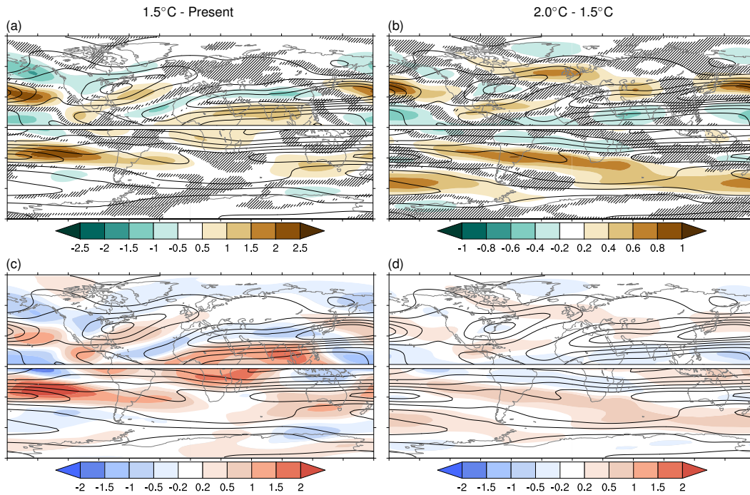
Figure 5. Multi-model mean response of winter (Northern Hemisphere DJF, Southern Hemisphere JJA) zonal wind at 250 hPa ( u_{250} ) for 1.5°C–PD (left) and 2.0°C–1.5°C (right). Top panels show responses (shading; units \text{m s}^{-1} ) along with the climatology (contour interval 10 \text{ m s}^{-1} ) for the (a) PD and (b) 1.5°C experiments. Note the different colour scale for (a) and (b). Bottom panels show signal-to-noise ratio \beta/\sigma , where the sign corresponds to the sign of the response, along with the climatology (contour interval 10 \text{ m s}^{-1} ) for the (c) 1.5°C and (d) 2.0°C experiments. In (a) and (b), hatching masks out regions where there is no model consensus (fewer than four out of five models agree) on the sign of the response. In (c) and (d), black dots mask out regions where the models do not agree on the magnitude of the response ( f^2 > 1 ).
