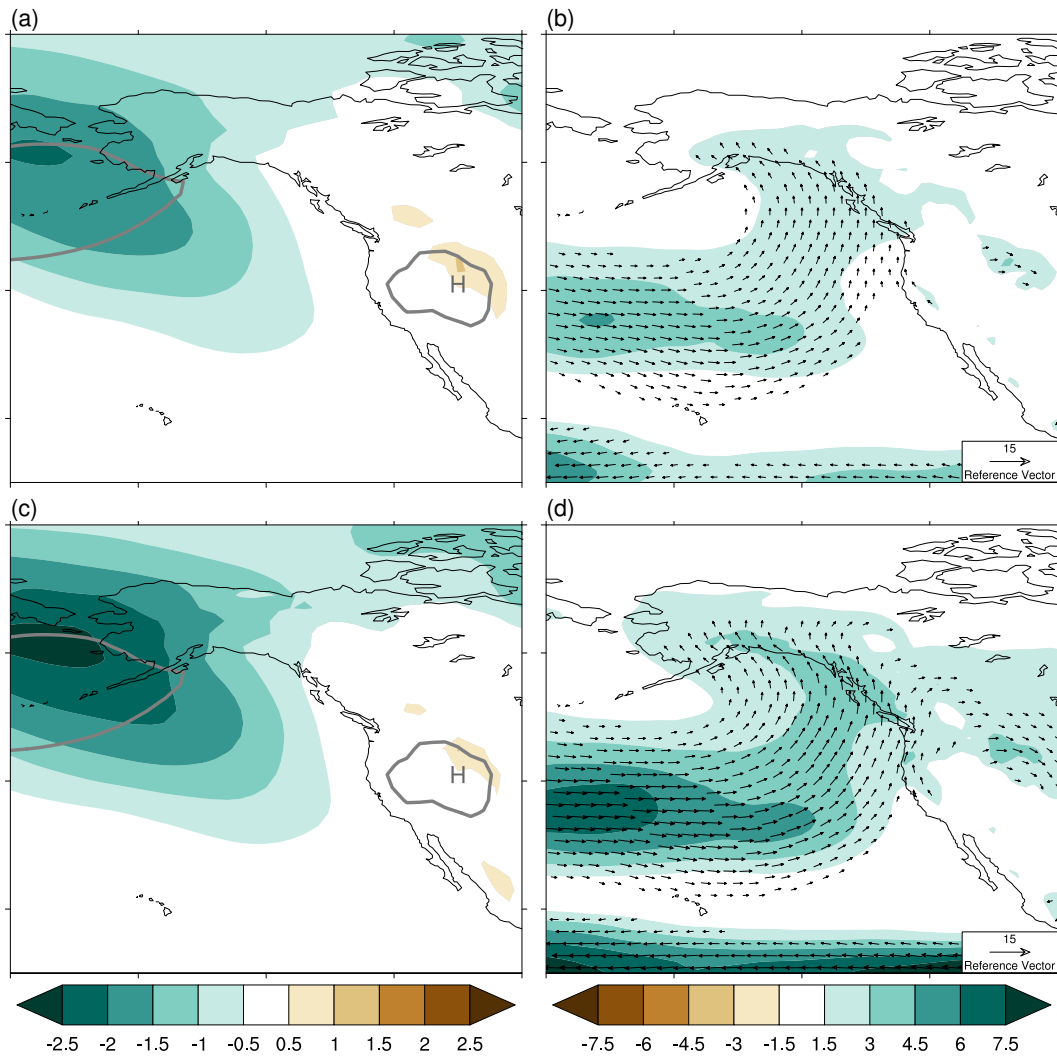
Figure 16. Wintertime (DJF) response of sea level pressure and moisture flux in (a,b) 1.5°C and (c,d) 2.0°C relative to PD in NorESM1-Happi. (a,c) MSLP response (shading; units hPa) along with the climatological 1000 hPa and 1025 hPa isobars from the PD experiment (grey contours). (b,d) 850-hPa specific humidity flux response (shading and vectors; units \text{g kg}^{-1} \text{m s}^{-1} ). Only vectors with magnitude greater than 2 \text{ g kg}^{-1} \text{m s}^{-1} are plotted.
