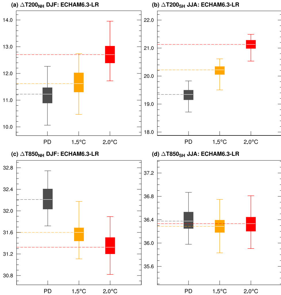
Figure 11. Changes in upper and lower level equator-to-pole temperature gradients (following Harvey et al., 2014) in the PD (grey), 1.5°C (orange) and 2.0°C (red) experiments in the ECHAM6.3-LR ensemble. The Northern Hemisphere temperature gradient is defined as the difference between the area-averaged temperature in the 30°S–30°N band and the region poleward of 60°N, taken at 850 hPa ( \Delta T_{850_{NH}} ) and 200 hPa ( \Delta T_{200_{NH}} ). The Southern Hemisphere gradient is defined as the the difference between the 30°S–30°N band and the region poleward of 60°S, taken at 850 hPa ( \Delta T_{850_{SH}} ) and 200 hPa ( \Delta T_{200_{SH}} ). The white horizontal line in the boxes indicates the median, the boxes indicate the interquartile range, and the whiskers indicate the ECHAM6.3-LR ensemble spread.
