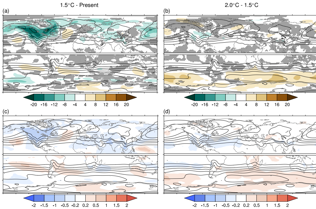
Figure 8. Multi-model mean response of winter (Northern Hemisphere DJF, Southern Hemisphere JJA) low-level MSLP storm tracks for 1.5°C–PD (left) and 2.0°C–1.5°C (right). Top panels show responses (shading; units hPa) along with the climatology (contour interval 100 hPa) for the (a) PD and (b) 1.5°C experiments. Bottom panels show signal-to-noise ratio \beta/\sigma , where the sign corresponds to the sign of the response, along with the climatology (contour interval 100 hPa) for the (c) 1.5°C and (d) 2.0°C experiments. In (a) and (b), hatching masks out regions where there is no model consensus (fewer than four out of five models agree) on the sign of the response. In (c) and (d), black dots mask out regions where the models do not agree on the magnitude of the response ( f^2 > 1 ). The storm tracks are defined as the standard deviation of bandpass filtered daily MSLP.
