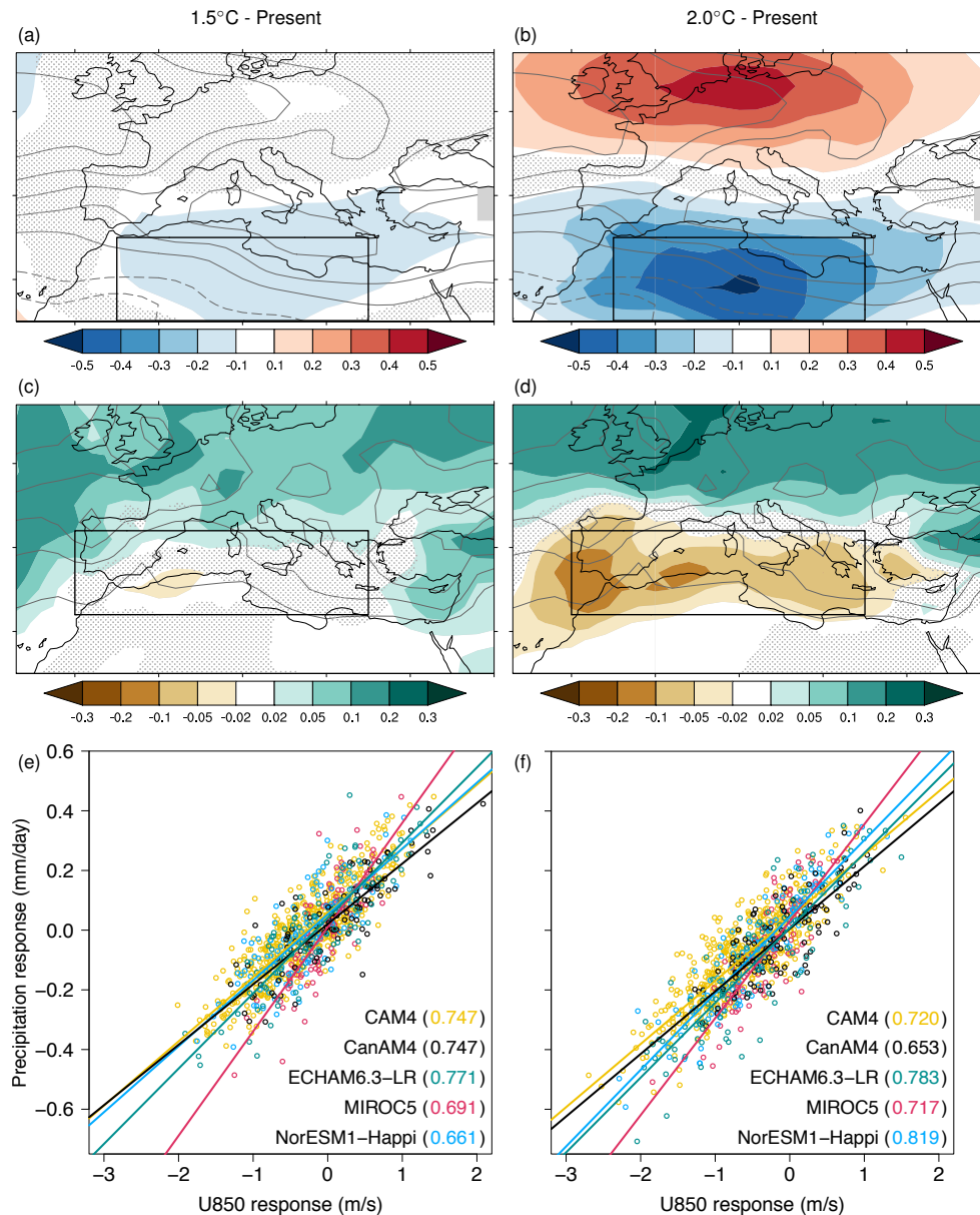
Figure 12. Multi-model mean winter (DJF) response of (a-b) zonal wind at 850 hPa and (c-d) precipitation in the 1.5°C (left) and 2.0°C (right) experiments relative to PD. Top panels show the multi-model mean responses (shading) and the PD climatology (contour interval 2 \text{ m s}^{-1} , dashed contours for negative values, zero contour omitted) for u_{850} . Middle panels show the multi-model mean responses (shading) and the PD climatology (contour interval 1 \text{ mm d}^{-1} ) for precipitation. Stippling in (a) to (d) masks out regions where the response is very weak (signal-to-noise ratio |\beta/\sigma| < 0.1 ). Bottom panels show the relationship between the area-averaged precipitation and u_{850} responses in the (e) 1.5°C and (f) 2.0°C experiments relative to PD, with the R^2 value for each model indicated in the legend. Boxes in the maps indicate the regions used for calculating area-averaged responses.
