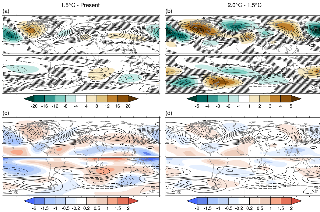
Figure 10. Multi-model mean response of winter (Northern Hemisphere DJF, Southern Hemisphere JJA) stationary waves at 500 hPa for 1.5°C–PD (left) and 2.0°C–1.5°C (right). Top panels show responses (shading; units m) along with the climatology (contour interval 25 m) for the (a) PD and (b) 1.5°C experiments. Note the different colour scale for (a) and (b). Bottom panels show signal-to-noise ratio \beta/\sigma , where the sign corresponds to the sign of the response, along with the climatology (contour interval 25 m) for the (c) 1.5°C and (d) 2.0°C experiments. In (a) and (b), hatching masks out regions where there is no model consensus (fewer than four out of five models agree) on the sign of the response. In (c) and (d), black dots mask out regions where the models do not agree on the magnitude of the response ( f^2 > 1 ). Stationary waves are defined as departures from the zonal mean of geopotential height ( Z^* ) at 500 hPa.
