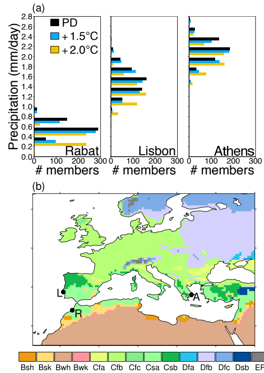
Figure 14. (a) Histograms of decadal mean winter (DJF) precipitation in Rabat, Lisbon and Athens for the PD, 1.5°C and 2.0°C experiments from the CAM4 ensemble. The locations are indicated in panel b as well as in Figure 13 . (b) Climate zones according to the Köppen-Geiger classification scheme (Kottek et al., 2006). The Mediterranean is primarily a temperate zone with dry summers (Csa, Csb), but includes some arid regions (Bsk, BSh).
