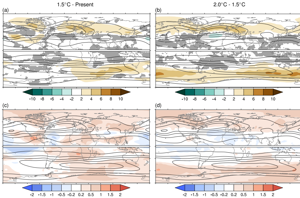
Figure 9. Multi-model mean response of winter (Northern Hemisphere DJF, Southern Hemisphere JJA) upper level EKE storm tracks for 1.5°C–PD (left) and 2.0°C–1.5°C (right). Top panels show responses (shading; units \text{m}^2 \text{s}^{-2} ) along with the climatology (contour interval 40 \text{ m}^2 \text{s}^{-2} ) for the (a) PD and (b) 1.5°C experiments. Bottom panels show signal-to-noise ratio \beta/\sigma , where the sign corresponds to the sign of the response, along with the climatology (contour interval 40 \text{ m}^2 \text{s}^{-2} ) for the (c) 1.5°C and (d) 2.0°C experiments. In (a) and (b), hatching masks out regions where there is no model consensus (fewer than four out of five models agree) on the sign of the response. In (c) and (d), black dots mask out regions where the models do not agree on the magnitude of the response ( f^2 > 1 ). The storm tracks are defined as EKE calculated from bandpass filtered daily wind at 250 hPa.
