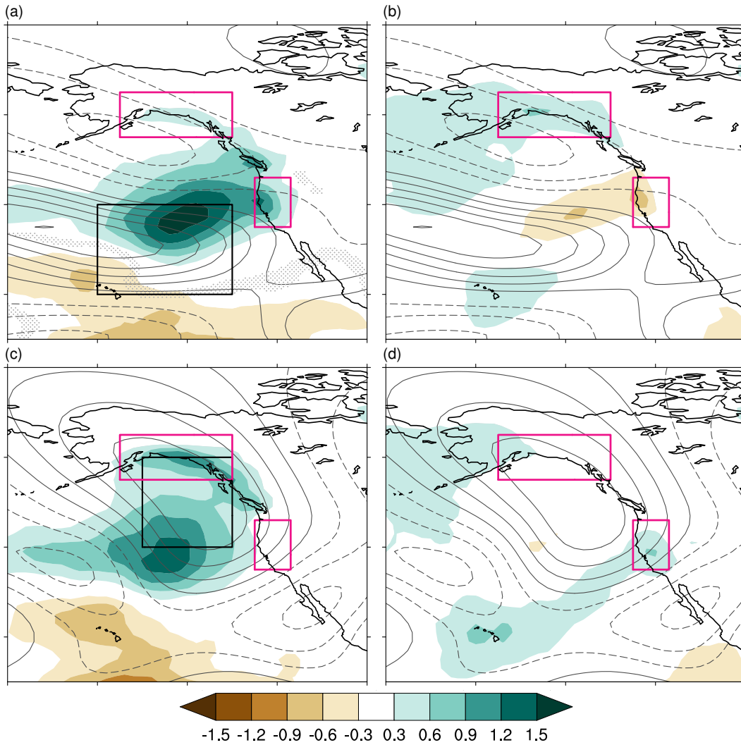
Figure 17. Multi-model mean precipitation signals associated with wind changes over western North America in the 2.0°C experiment during winter (DJF). Top: Composites of precipitation (units: \text{mm day}^{-1} ) based on westerly u_{250} changes in the North Pacific jet exit (area indicated in (a) by southern the black box), over members with the (a) 5% strongest and (b) 5% weakest westerly responses. Contours show the u_{250} climatology (contour interval 0.5 \text{ m s}^{-1} , zero contour omitted) for the PD experiment. Bottom: Composites of precipitation (units: \text{mm day}^{-1} ) based on southerly v_{250*} changes off the coast (area indicated in (a) by northern the black box), over members with the (c) 5% strongest and (d) 5% weakest southerly responses. Contours show the v_{250*} climatology (contour interval 0.4 \text{ m s}^{-1} , zero contour omitted) for the PD experiment, where v_{250*} is the departure from the zonal mean of the meridional wind at 250 hPa.
