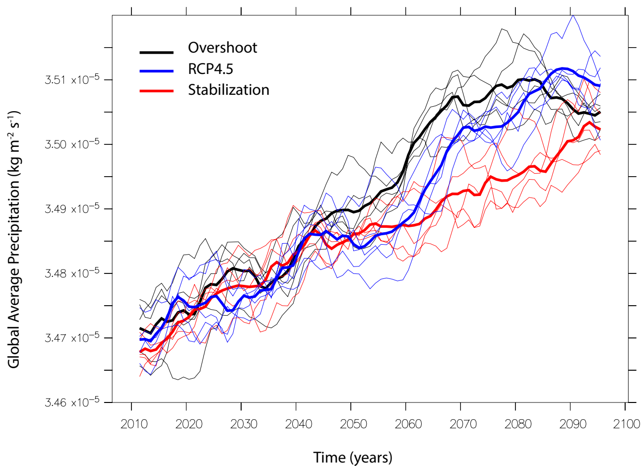
Supplementary Figure S2: Globally averaged precipitation (kg m -2 s -1 ) for the Stabilization (red), Overshoot (black), and RCP4.5 (blue) scenarios. The bold lines are ensemble means and the thin lines are individual ensemble members.
