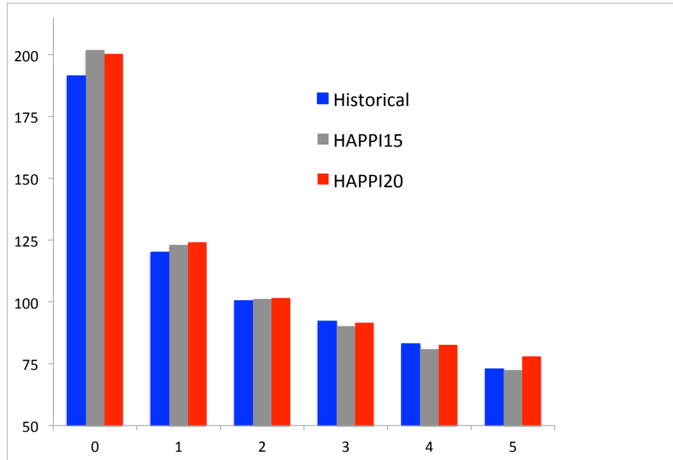
Figure 8. Chavas radii at different wind speeds selected as the definitions of the Saffir-Simpson categories (km) for the HAPPI simulations. Blue: Historical. Gray: 1.5° Stabilization. Red: 2.0° Stabilization.
