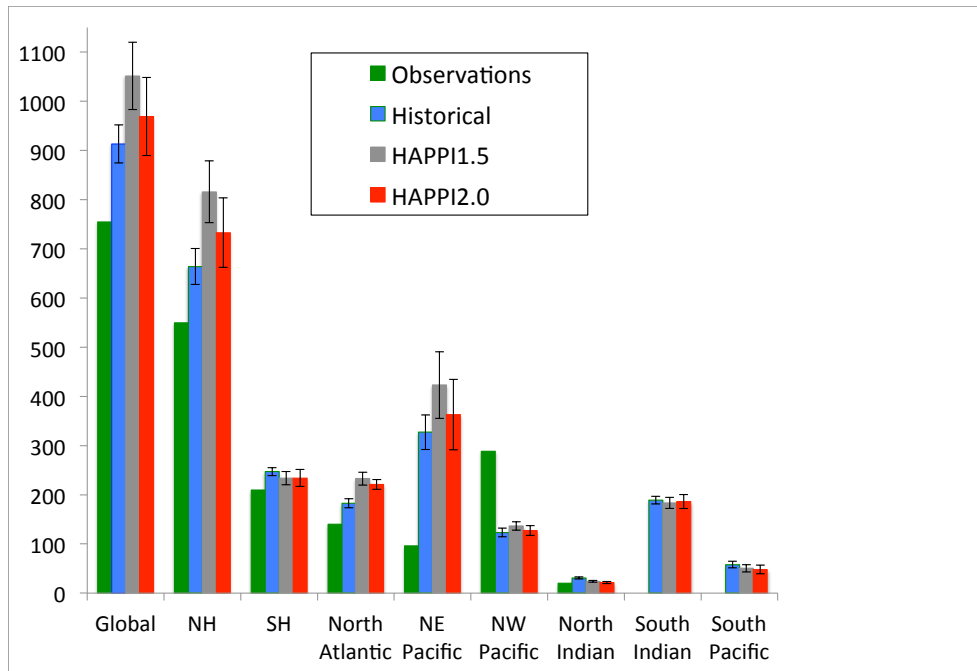
Figure 6. Average annual Accumulated Cyclonic Energy (ACE) for the Historical and HAPPI stabilization scenarios for all named storms by basin and globally for intense tropical cyclones only. Units: 1 ACE=10 4 knots. Green: Observations. Blue: Historical. Gray: 1.5° Stabilization. Red: 2.0° Stabilization. Error bars are standard errors based on interannual variability.
