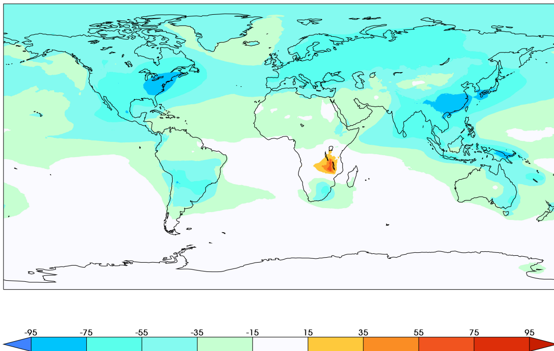
Figure 2: Percent difference between the stabilized 2°C scenario and the historical simulation of the total aerosol optical depth in the visible band.
