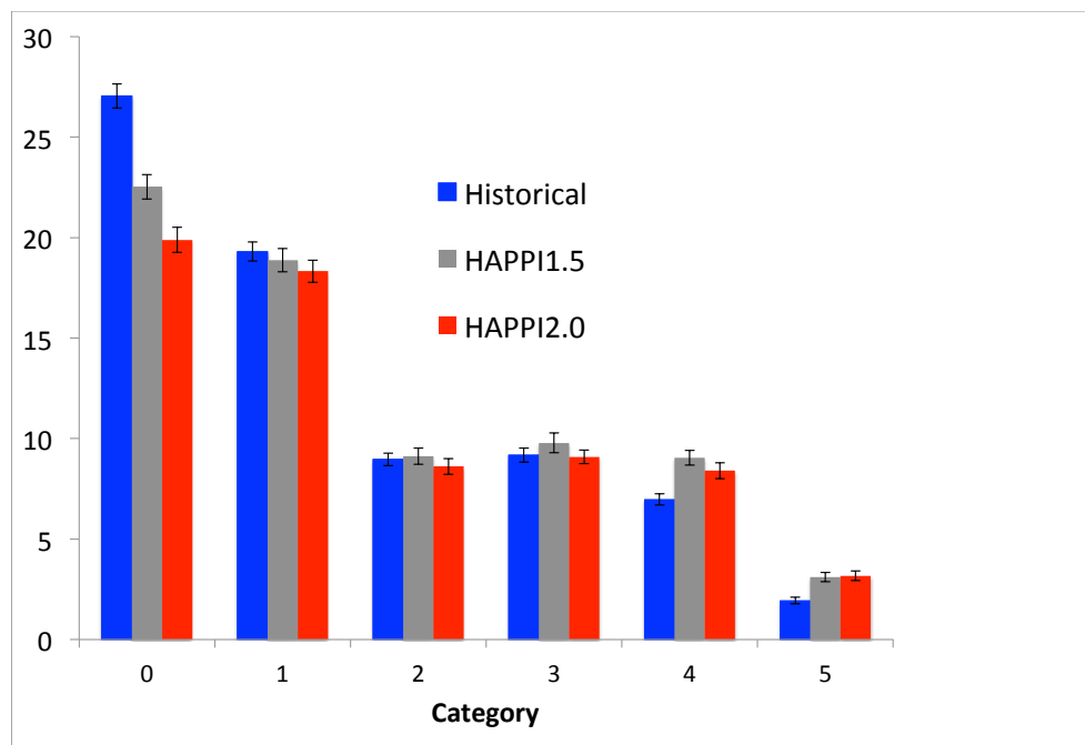
Figure 3. Global annual number of tropical cyclones by Saffir-Simpson scales for the historical (blue), 1.5°C stabilization scenario (gray), 2°C stabilization scenario (red).
