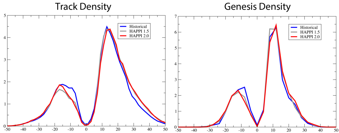
Figure 5. Left: Zonally averaged normalized tropical storm track density for the HAPPI scenarios. Right: Zonally averaged normalized tropical storm genesis density for the HAPPI scenarios. Blue: Historical. Gray: 1.5° Stabilization. Red: 2.0° Stabilization.
