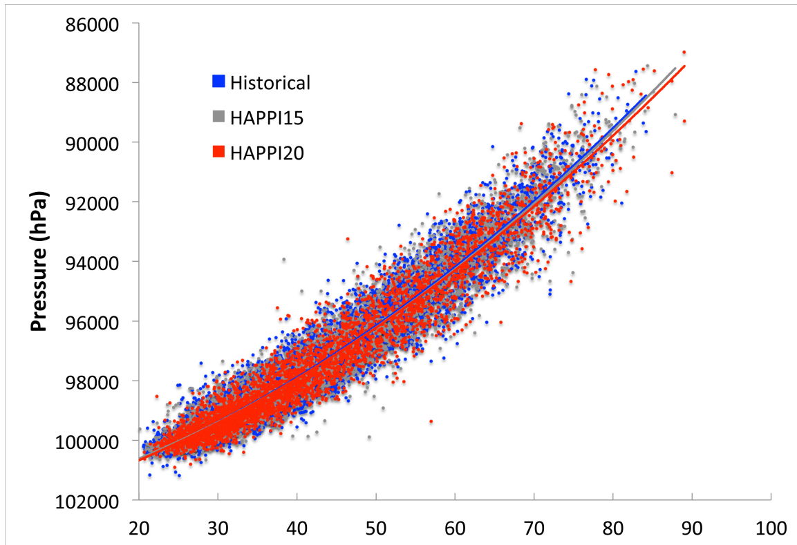
Figure 7: Scatterplot of minimum central pressure (hPa) versus maximum wind speed (m/s) at the time of maximum intensity for the HAPPI simulations. Blue: Historical. Gray: 1.5° Stabilization. Red: 2.0° Stabilization. Solid lines are quadratic fits to the data.
