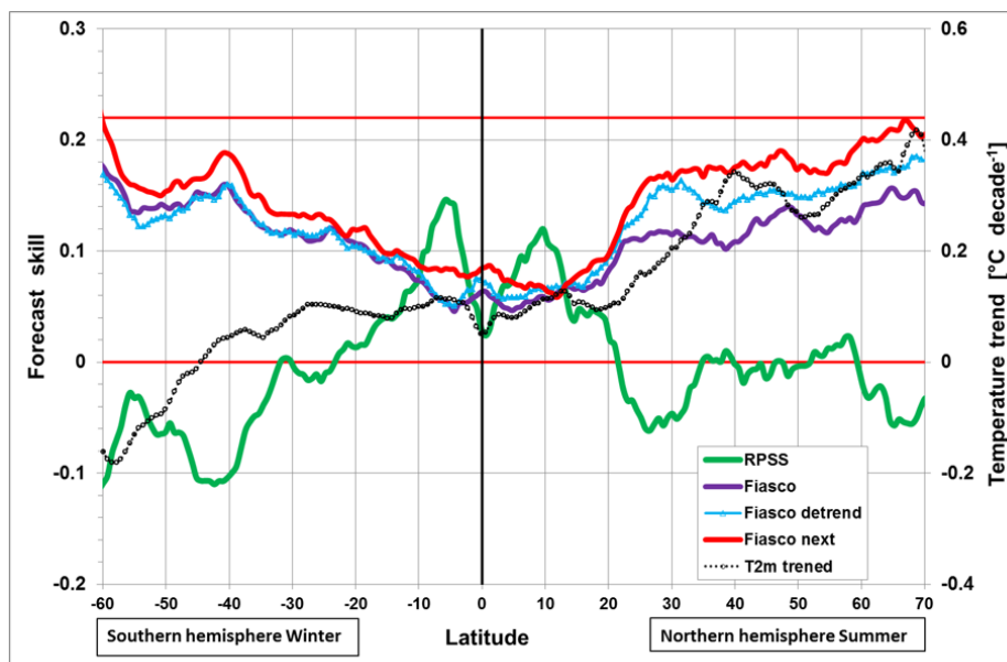
Fig. 1. The latitude average over sea and land of ECMWF Sys4 hindcast (1981-2010) Rank Probability Score Skill (RPSS), the "Fiasco score", the "Fiasco score" after de-trending and the "Fiasco next score" of t
