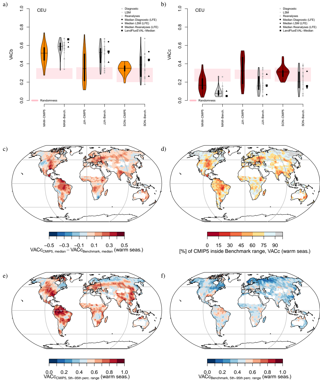
Figure 2. Evaluation of T-ET coupling in global climate models. (a, b) VAC b (a) and VAC c coupling in the CMIP5 climate model ensemble and observations-based benchmarking datasets in Central Europe (CEU, 1989-2005, area-average) with systematic warm season differences. Randomness indicates the 5th to 95th percentile range obtained by randomly permutating both time series with respect to the other ( N = 100 times) to obtain independent data. (c) Difference in the VAC c median of the CMIP5 ensemble and benchmarking datasets. (d) Fraction of CMIP5 models that are inside the 5th-95th percentile spread of the benchmarking datasets. (e, f) Range of VAC c -occurrences (5th to 95th percentile range) in CMIP5 models (e) and in the ensemble of observations (f).
