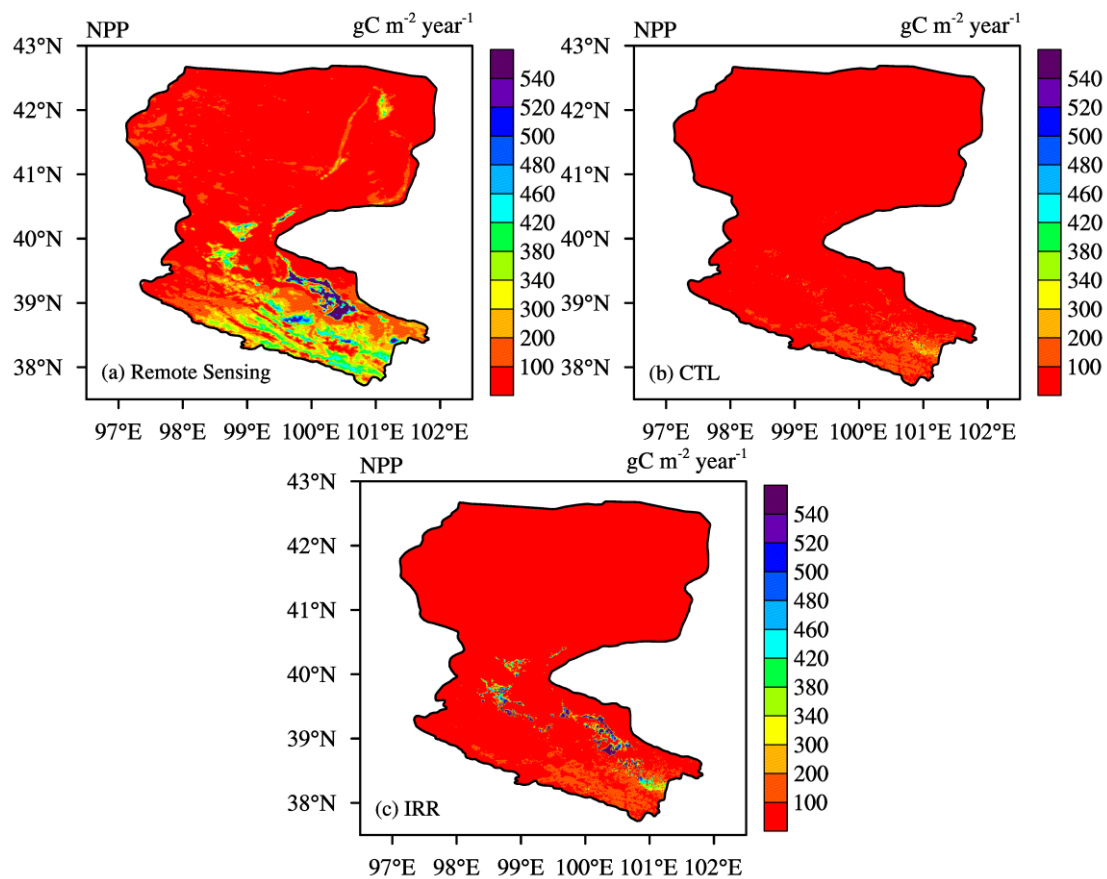
Figure 6: Climatologic NPP distribution from 1998 to 2002 over Heihe River Basin obtained from (a) remote sensing, (b) CTL and, (c) IRR.
