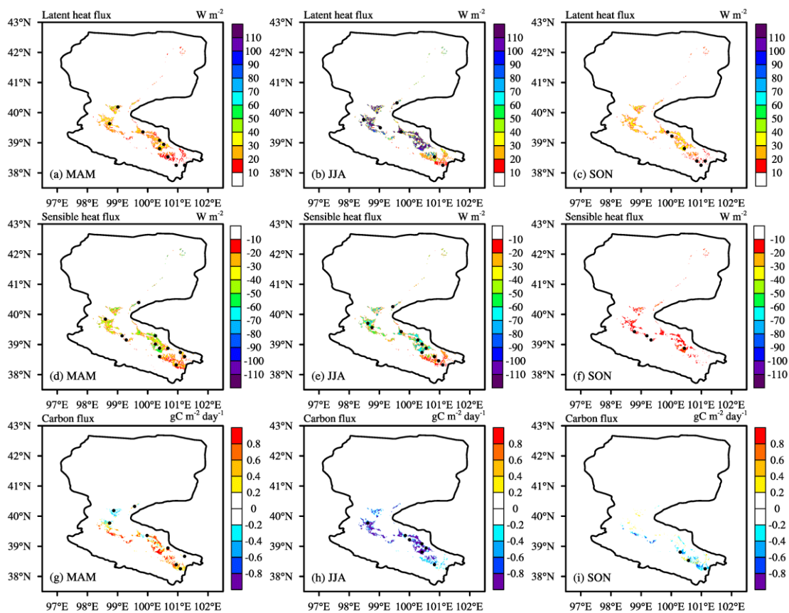
Figure 7: Climatic spatial pattern of (a-c) latent heat flux, (d-f) sensible heat flux and (g-i) carbon flux differences between IRR and CTL in (a, d, g) spring, (b, e, h) summer and (c, f, i) autumn, averaged from 1981 to 2013. The dots represent the area that passed the Student's t-test at a 95% confidence level.
