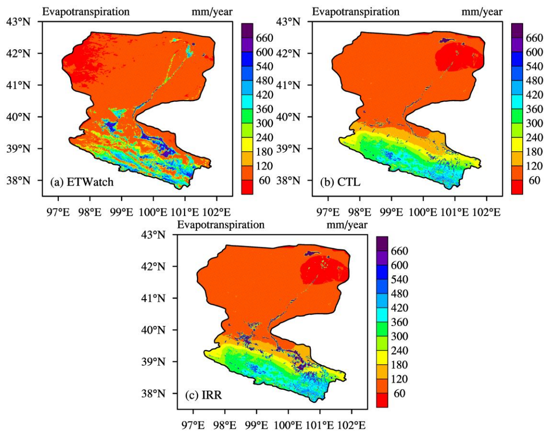
Figure 5: Climatologic evapotranspiration distribution from 2000 to 2003 over the Heihe River Basin obtained from (a) ETWatch (b) CTL and, (c) IRR.
