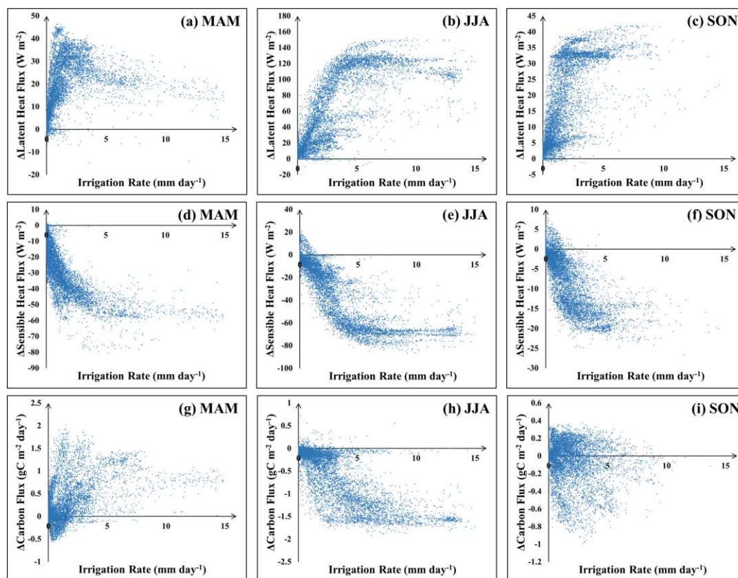
Figure 8: Differences of (a-c) latent heat flux, (d-f) sensible heat flux and (g-i) carbon flux between IRR and CTL models versus the irrigation rate in (a, d, g) spring, (b, e, h) summer and, (c, f, i) autumn.
