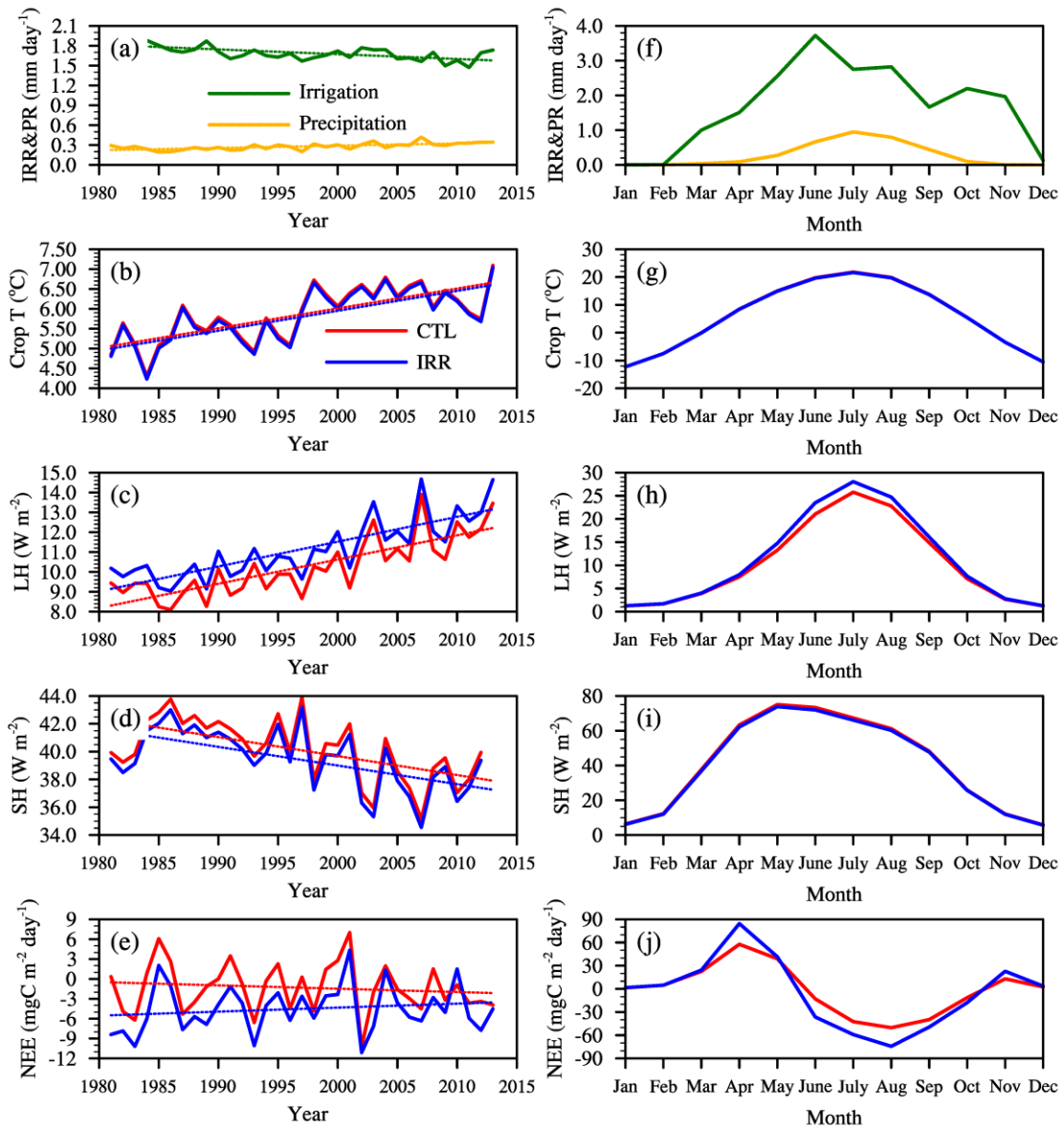
Figure 9: Time evolution plots of (a-e) annual and (f-j) seasonal (a, f) irrigation and precipitation, (b, g) crop temperature, (c, h) latent heat flux, (d, i) sensible heat flux and, (e, j) carbon heat flux, averaged over all crop grids of the Heihe River Basin.
