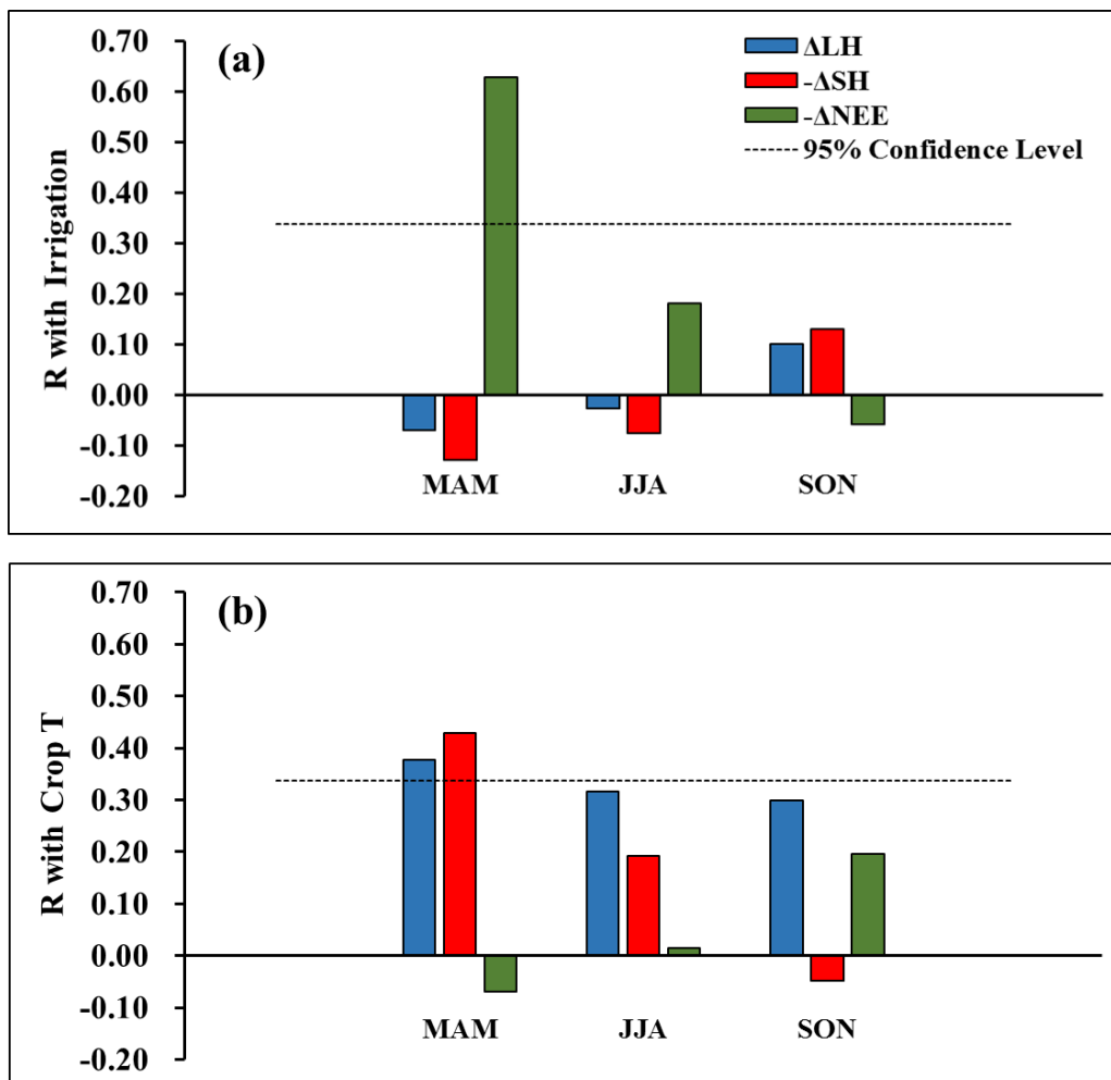
Figure 10: (a) Temporal correlation coefficients between the irrigation rate and \Delta LH , -\Delta SH , -\Delta NEE over the spring, summer and autumn and, (b) temporal correlation coefficients between the crop temperature and \Delta LH , -\Delta SH , -\Delta NEE over the spring, summer and autumn.
