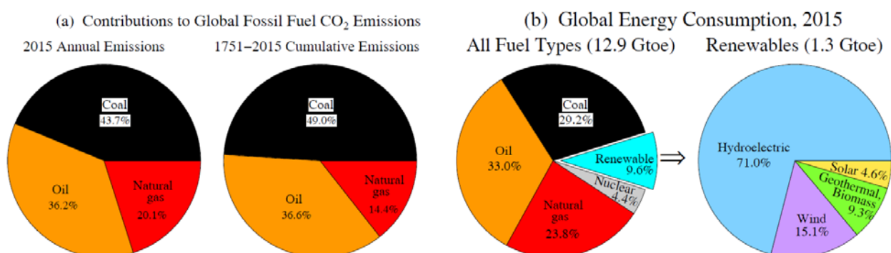
Figure 13. (a) Global fossil fuel emissions data from Boden et al. (2017) for 1751–2014 are extended to 2015 using BP (2016) data. (b) Global primary energy consumption data from BP (2016).
