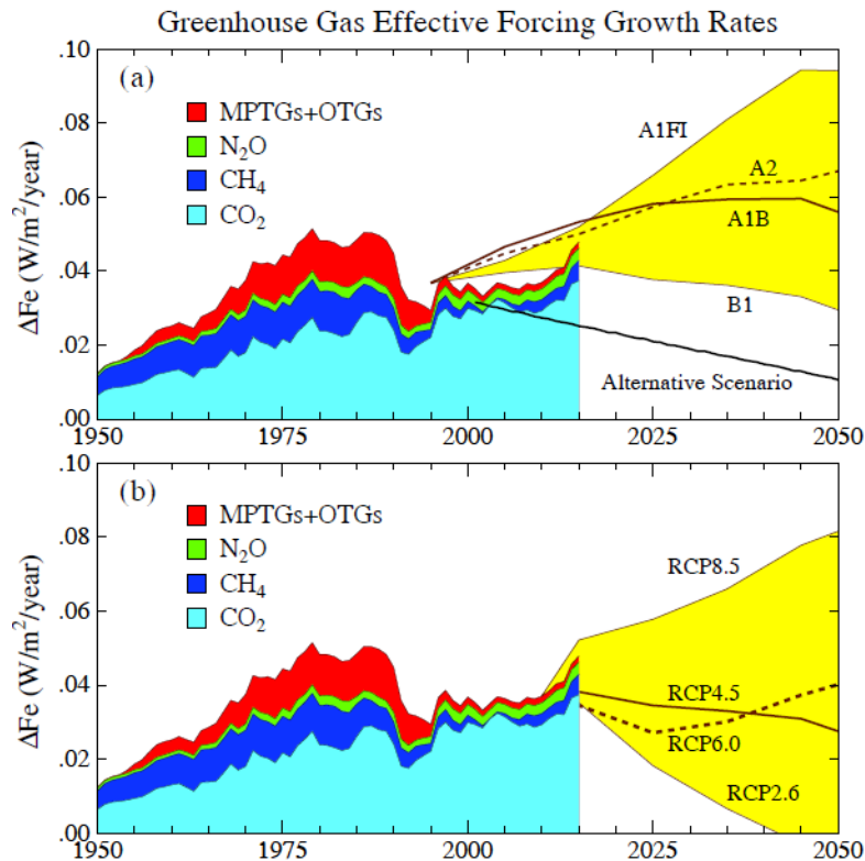
Figure 8. GHG climate forcing growth rate with historical data being 5-year running means, except data for 2015 are a 3-year mean. (a) includes scenarios used in IPCC AR3 and AR4 reports, and (b) has AR5 scenarios. GHG amounts are from NOAA/ESRL Global Monitoring Division. O 3 changes are not fully included, as they are not well-measured, but its tropospheric changes are partially included via the effective CH 4 forcing. Effective climate forcing, MPTGs and OTGs are as defined in Fig. 4 caption.
