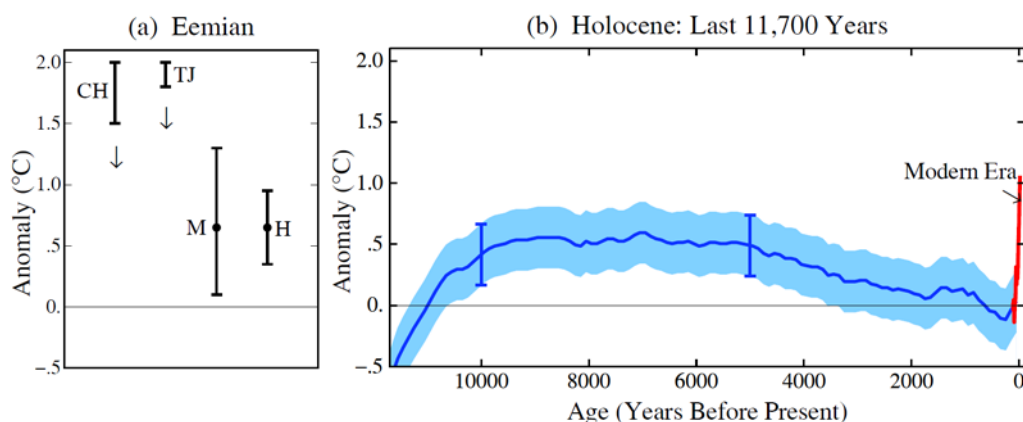
Figure 3. Estimated average global temperature for (a) last interglacial (Eemian) period (Clark and Huybers, 2009; Turney and Jones, 2010; McKay et al., 2011; Hoffman et al., 2017), (b) centennially-smoothed Holocene (Marcott et al., 2013) temperature and the 11-year mean of modern data (Fig. 2), as anomalies relative to 1880-1920. Vertical downward arrows indicate likely overestimates (see text).
