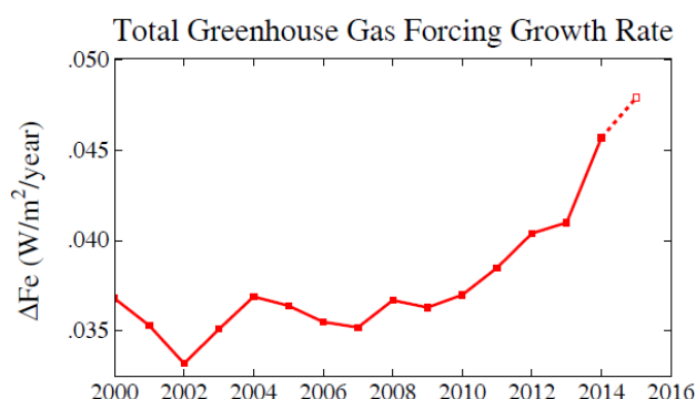
Figure 14. Recent growth rate of total GHG climate forcing; points are 5-year running means, except 2015 point is a 3-year mean. See Fig. 8 for individual gases.
