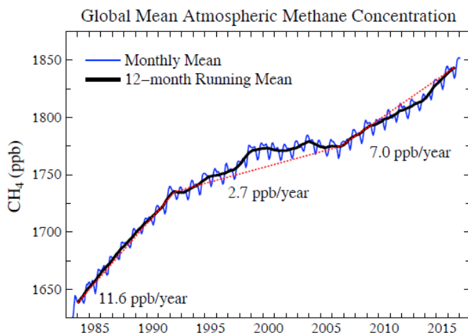
Figure 7. Global CH 4 from Dlugokencky (2016), NOAA/ESRL ( www.esrl.noaa.gov/gmd/ccgg/trends_ch4/ ). End months for three indicated slopes are January 1984, May 1992, August 2006, and January 2017.
