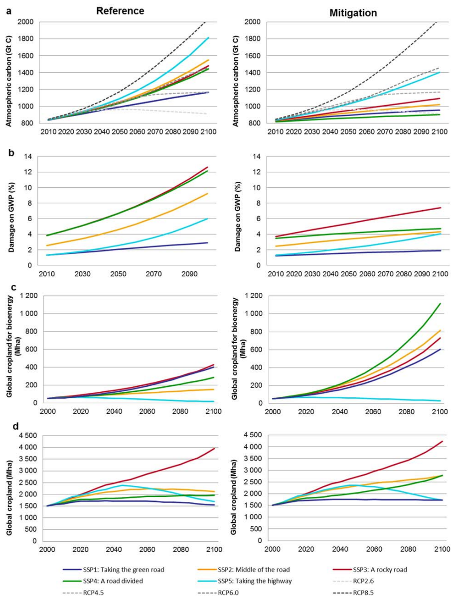
Figure 4. (a) Atmospheric carbon (GtC) including carbon trajectories (GtC) for the four RCPs, (b) corresponding damage to GWP (%), (c) global cropland for bioenergy (Mha) and (d) global cropland (Mha) for reference and mitigation scenarios.
