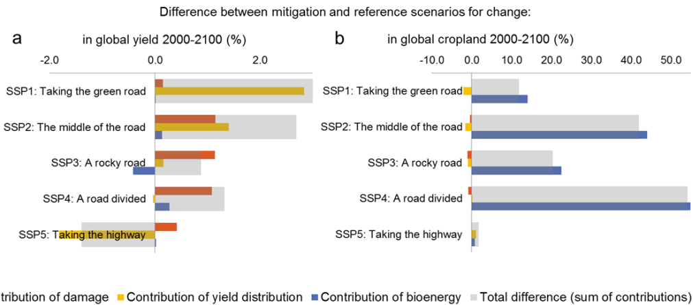
Figure 6. (a) Difference between reference and mitigation scenarios for change in global yield between 2000 and 2100 (%) and (b) change in global cropland area between 2000 and 2100 (%). The grey bar gives the total differences (sum of differences due to damage, yield distribution and bioenergy), while the colored bars show the contribution of each causal factor to the total difference.
