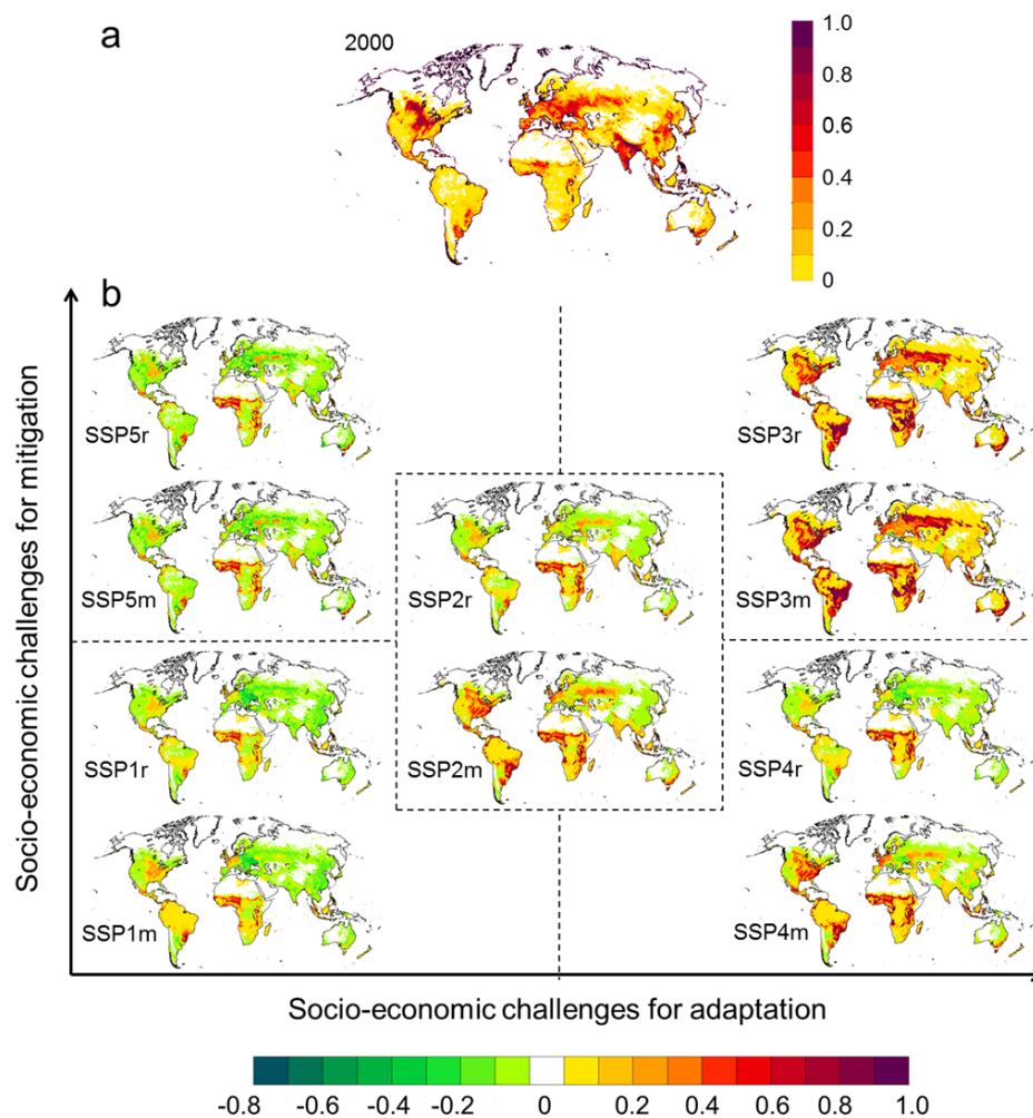
Figure 7. (a) Fraction of cropland on total land area for baseline year 2000 based on Hurtt et al. (2011). (b) Simulated cropland changes relative to baseline by 2100 for the five SSP reference (r) and mitigation (m) scenarios in the challenge for adaptation and mitigation space. Green colours indicate a decrease in cropland area in 2100 compared to 2000, while yellow and red colours indicate an increase in cropland area in 2100 compared to 2000.
