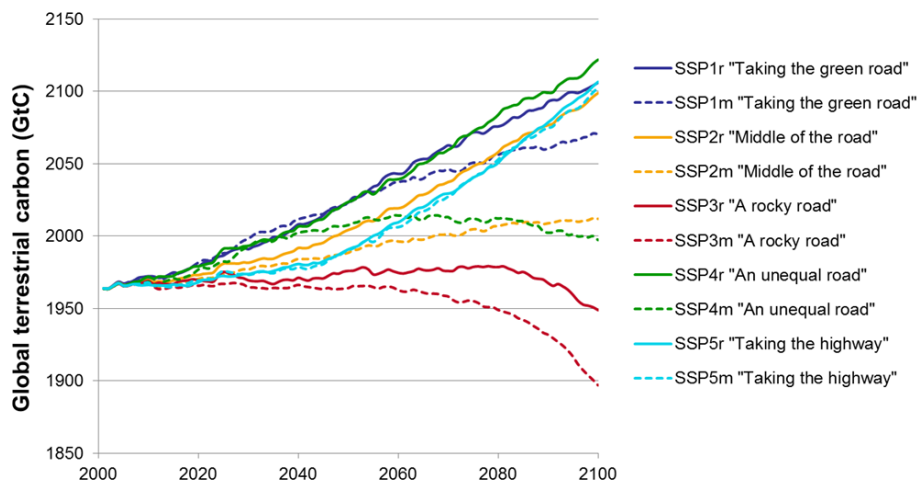
Figure 9: Changes in global terrestrial biosphere carbon pool (GtC) from 2000 to 2100 for all SSPs, reference (r) and mitigation (m) case. The slope indicates whether the net ecosystem carbon balance (NECB) is a carbon source (negative slope) or carbon sink (positive slope).
