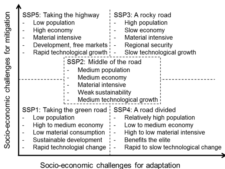
5 Figure 1. The SSP scenarios of global socio-economic development in the 21st century in their space of challenges for mitigation and adaption (adapted from O'Neill et al. 2013) and their development in selected key elements: growth of population, growth of the economy, lifestyle, policy orientation and technological development (O'Neill et al., in press).
