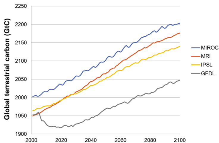
5 Figure A 2: Global terrestrial biosphere carbon (GtC) simulated with climate forcing fields from four GCMs (MIROC (Watanabe et al. 2010), MRI (Yukimoto et al. 2012), IPSL (Dufresne et al., 2013) and GFDL (Donner et al., 2011) for medium LULCC (SSP2m) and RCP4.5 driven climate change. Uncertainties due to different process representations in the four GCMs arrive at differences across the GCMs in 2100 which are similar to the total simulated change for one GCM (e.g. difference MIROC-GFDL is around 150 GtC in 2100, while total simulated change of GFDL is around 100 GtC or 200 for MIROC). The initial dip in GFDL terrestrial carbon is mainly caused by Amazon forest dieback.
