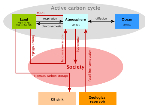
Figure 1. Structure of the co-evolutionary model of societal monitoring and tCDR intervention in the carbon cycle including simulated components of the carbon cycle as well as a societal management loop and their interactions. Carbon values in the boxes indicate estimates of preindustrial carbon pools in the year 1750 AD (Batjes, 1996; Ciais et al., 2013)).
