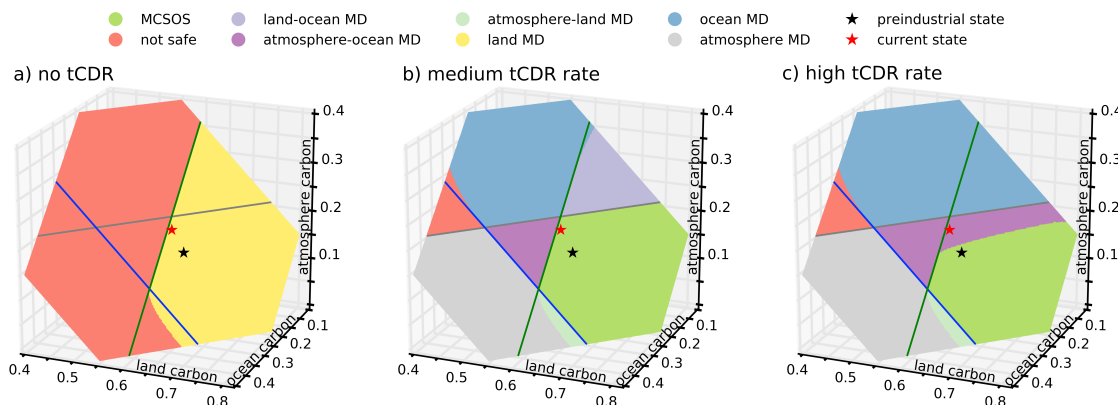
Figure 6. Charting of normalised carbon system state space in our model for three tCDR management characteristics with identical, relatively low emission baseline ( c_{max} = 0.2 ): a) without tCDR ( \alpha_{max} = 0 ), b) intermediate tCDR rates ( \alpha_{max} = 0.004 ) and c) high tCDR rates ( \alpha_{max} = 0.04 ). The two-dimensional plane is formed by sampling initial conditions around the preindustrial state (variation of carbon stocks by \pm 0.2 while conserving total carbon in the system). Each domain is coloured according to transient properties of trajectories starting in different state space regions. For example, the MCSOS (i.e. safe domain) is formed by the initial conditions of safe trajectories, whereas red indicates the initial conditions of trajectories crossing all respective planetary boundaries at some point of the simulation. Lines indicate the associated planetary boundaries of atmosphere, land and ocean in grey, green and blue, respectively.
