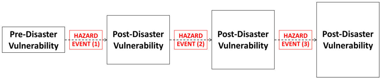
Figure 8. Example of vulnerability changes during-within a network of hazard interactions (cascade). A representation of changing vulnerability during a hazard cascade, where the magnitude of vulnerability is proportional to the size of the box. Following a disaster event, pressures on society, infrastructure and coping capacity are likely to be increased, and thus the vulnerability of a community and its systems/assets to further shocks or hazards may increase.
