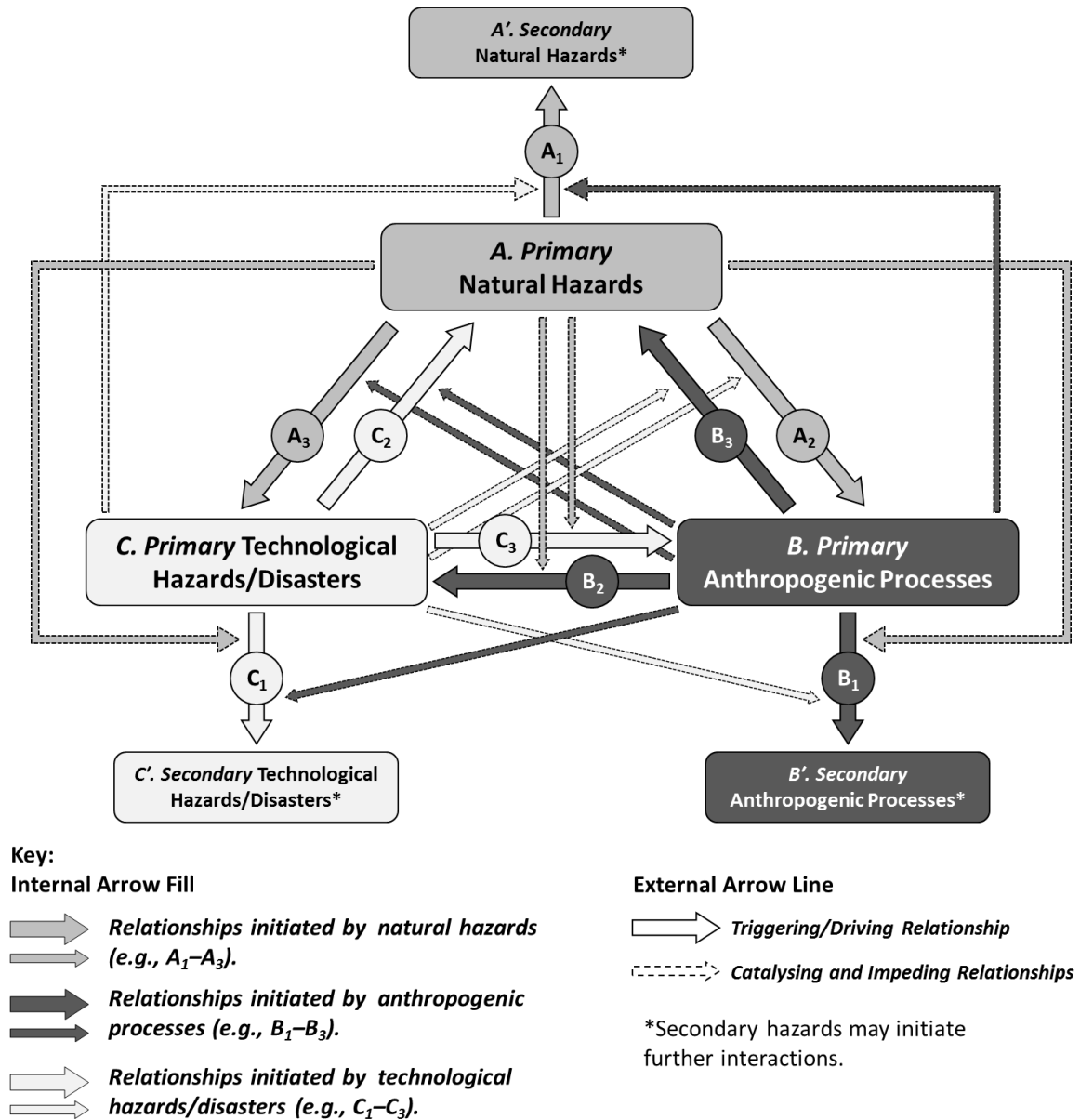
Figure 3. Interaction relationships (triggering, catalysing and impeding) framework using a hazard/process flow diagram. Interactions in the form of triggering relationships ( Figure 2 ), and catalysing/impedance interactions are possible between ( A ) natural hazards, ( B ) anthropogenic processes and ( C ) technological hazards/disasters. We use a prime ( A' , B' , C' ) to indicate secondary hazards/processes triggered by the same primary hazard/process group ( A , B , C ). We contrast here triggering relationships (thick block arrows with solid outlines) and catalysing/impedance relationships (thin block arrows with dashed outlines). The internal arrow fill colour indicates the group of hazards or processes to which the catalyst/impeder belongs
