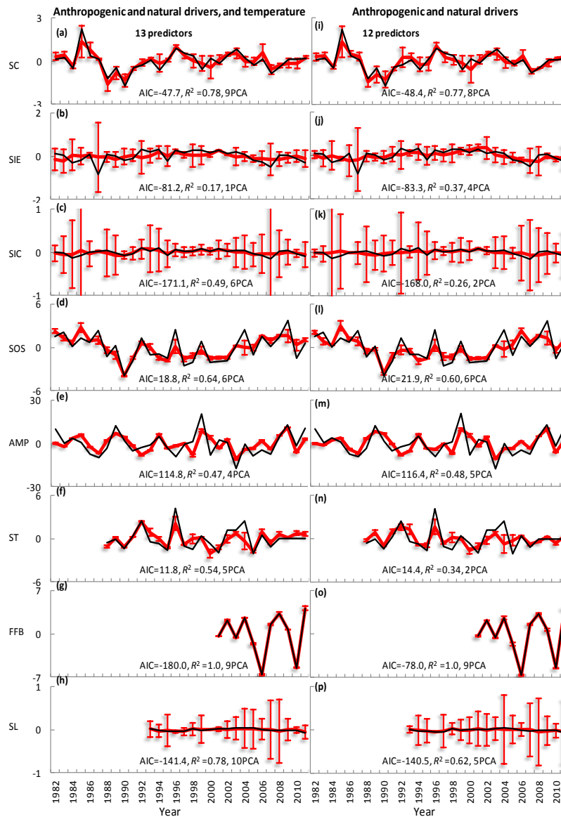
Figure 5. Predicting powers of temperature mediated natural and anthropogenic drivers (left), and only natural and anthropogenic drivers (right). Black line is observed and red line is predicted. Error bars are uncertainty of each prediction measured by standardized error. The predictions were conducted using stepwise regression with Akaike information criterion (AIC) from orthogonal variables transformed by principal component analysis (PCA) against each land, cryosphere and ocean indicator. The number of PCAs selected using the AIC criteria are shown in each panel. Predictors on left panels include the orthogonally transformed PCA variables of temperature, concentration (PPM) of atmospheric CO 2 at Point Barrow, 20 global well-mixed greenhouse gases (WMGHG) radiative forcing, solar radiation, sunspot numbers and eight leading Northern Hemisphere teleconnection indices. Panels on right include all the predictors on the left with exclusion of temperature. Each PCA for the two sets (i.e. left and right panels) were conducted separately.
