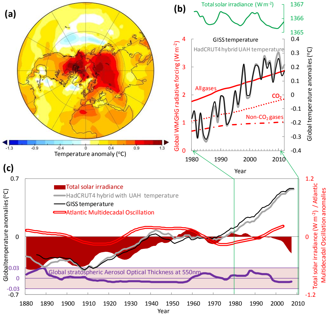
Figure 1. (a) 1980–2012 surface temperature anomaly (°C) of Northern Hemisphere relative to 1951–1980 base period. (b) The global mean annual surface temperature anomalies, total solar irradiance, and global well-mixed greenhouse gases (WMGHG) patterns during the satellite era. The WMGHG includes CO 2 , major gases (CH 4 , N 2 O, CFC12 and CFC11) and a set of 15 minor long-lived halogenated gases (CFC-113, CCl 4 , CH 3 CCl 3 , HCFCs 22, 141b and 142b, HFCs 134a, 152a, 23, 143a, and 125, SF 6 , and halons 1211, 1301 and 2402). Global annual mean surface temperatures relative to 1951–1980 base period from GISS (black) and Cowtan and Way HadCRUT4 hybrid UAH reconstruction (grey), and total solar irradiance are also shown in (b). (c) 11-year moving averages of global annual mean surface temperatures from GISS and Cowtan and Way HadCRUT4 hybrid UAH reconstruction, total solar irradiance, Atlantic Multidecadal Oscillation (AMO) index, and global stratospheric aerosol optical thickness at 550nm anomalies relative to 1951–1980 base period. The zoom-in arrows in (c) show the time period covered in this study when the temperature anomalies diverged from solar forcing and internal climatic variability.
