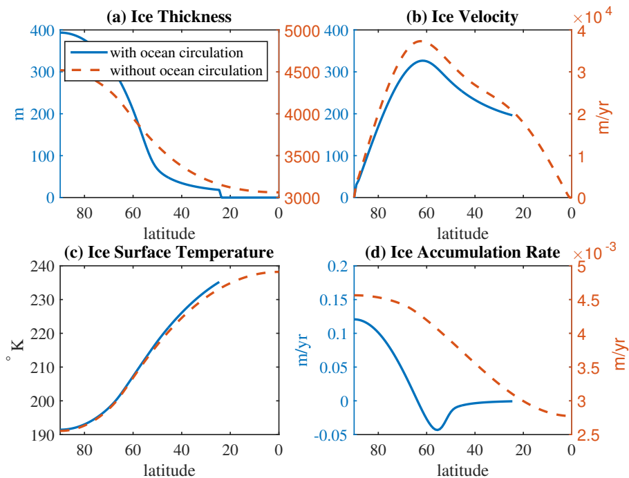
Figure 4. (a) Ice thickness h and (b) velocity v profiles with 94% insolation and \varepsilon = 0.82 , with and without ocean circulation. We note neglecting oceanic heat transport leads to drastically different global climate states. (c) Ice surface temperature T_s and (d) ice basal accumulation M , which without oceanic heat transport is positive everywhere.
