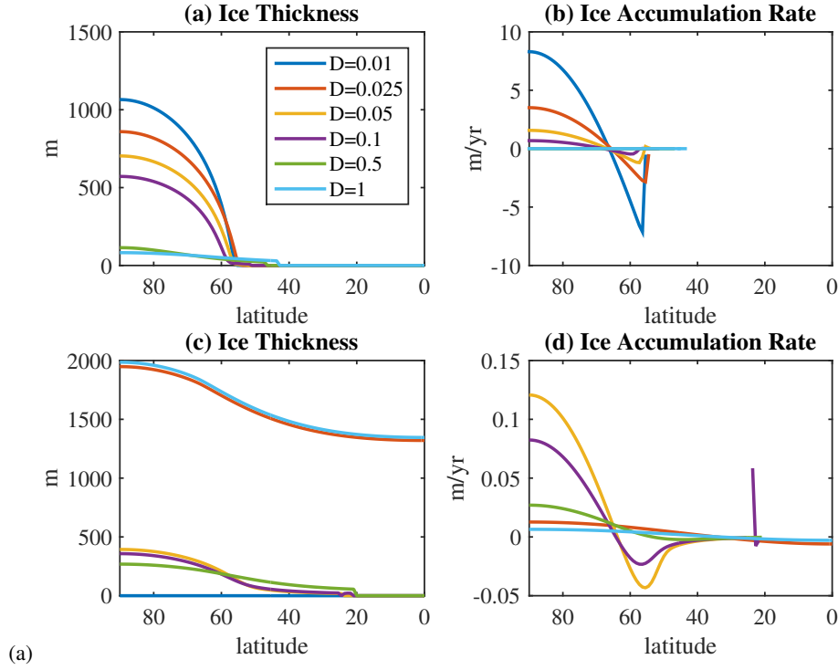
Figure 5. Effect of D parameter on equilibrium climate state, small ice cap regime ( \epsilon = 0.75 , top), and large ice cap regime ( \epsilon = 0.82 , 94% insolation, F_{geo} = 0.08W/m^2 bottom). There is particularly strong response in the resulting melting / accumulation term which was used to constrain the value of D . Furthermore, the instability near the large ice cap threshold is reflected in nearby values of D to the default D = 0.05 resulting in global ice cover for \epsilon = 0.82 .
