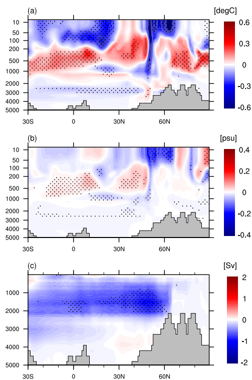
Fig. 5. Difference of (a) zonal mean ocean temperature, (b) zonal mean ocean salinity and (c) AMOC between experiments FE80 and FE-CTR (FE80 minus FE-CTR) for the Atlantic region.
