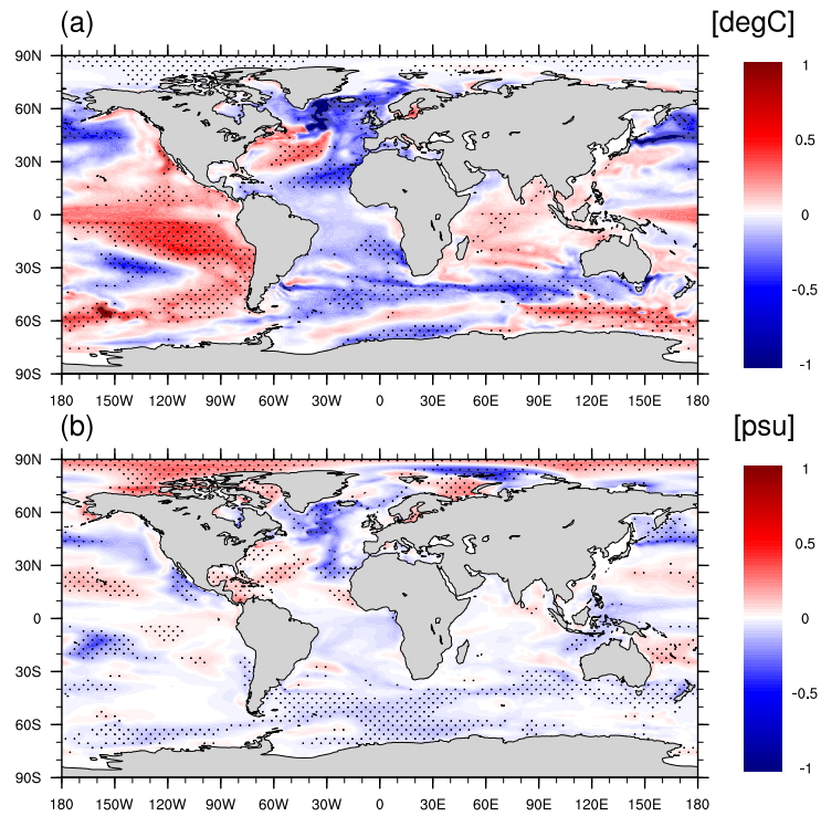
Fig. 3. Difference of annual mean (a) the sea surface temperature and (b) the sea surface salinity between experiments FE80 and FE-CTR (FE80 minus FE-CTR).
