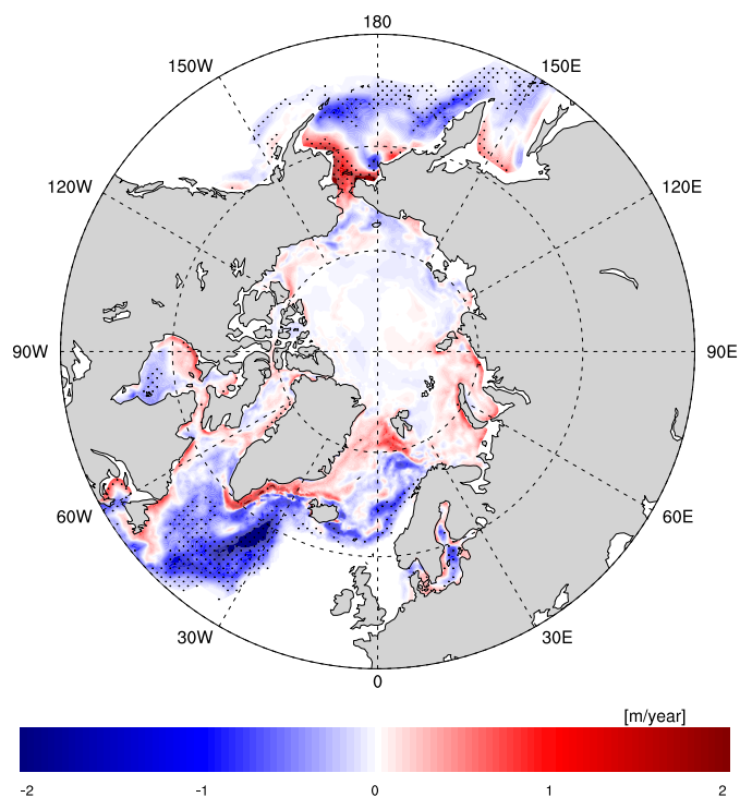
Fig. 4. Difference of annual mean thermodynamic growth rate of grid-cell mean ice thickness between experiments FE80 and FE-CTR (FE80 minus FE-CTR).
