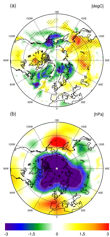
Fig. 6. Difference of (a) surface air temperature and (b) sea level pressure in boreal winter between experiments FE80 and FE-CTR (FE80 minus FE-CTR). Units are K and hPa.
