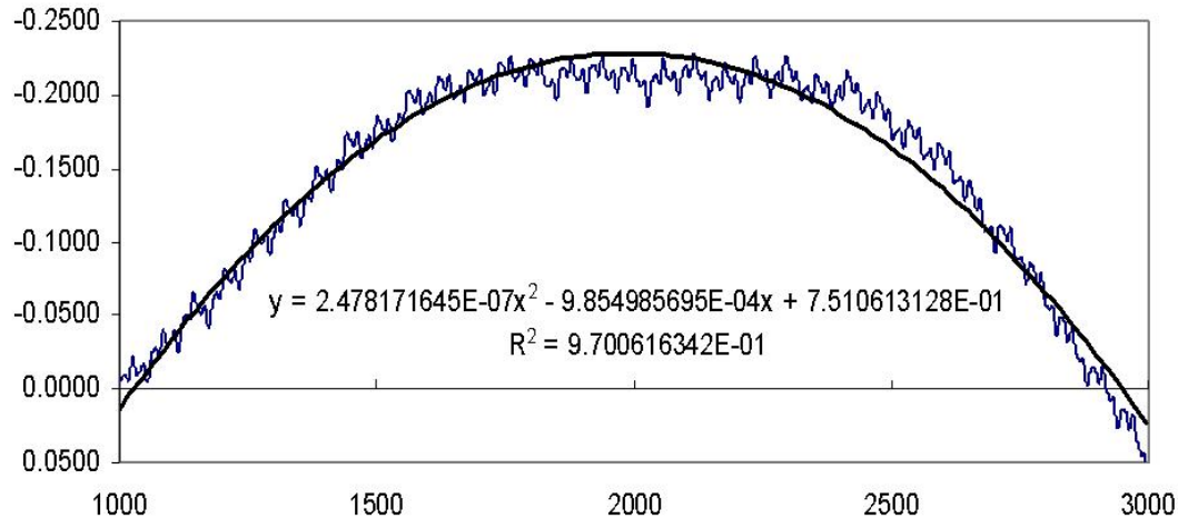
Figure C2.4. The double integral of the solar lateral inertial forces \sigma F_2(t) for the period from 1000 to 3000 AD. A polynomial trend is also depicted.
