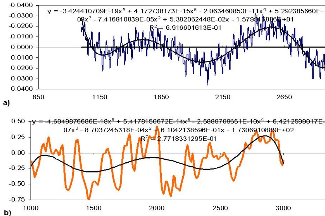
Figure C2.5. A comparison of the double integral of the solar lateral inertial forces \alpha \mathcal{F}_2(t) and the solar reconstructed and extrapolated record TSI. To enhance trends, polynomials are adjusted to both records, showing oscillations of \sim 950 and a lag of \sim 350 yrs.
