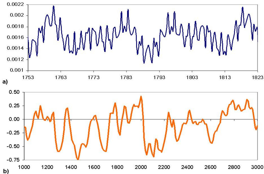
Figure C2.9. A comparison of the solar lateral forces F for the period from 1753 to 1823 AD, with the solar reconstructed and extrapolated record TSI for the period from 1000 to 3000 AD.
