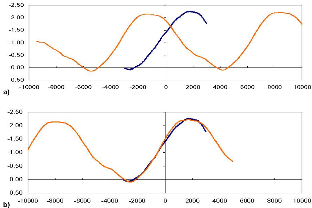
Figure C2.3. A comparison of the double integral of the solar lateral inertial forces \sigma_{F_2}(t) and the solar reconstructed and extrapolated record \sigma_{I_2}(t) . To enhance a possible cause-effect relationship |\sigma_{F_2}(t), \sigma_{I_2}(t) the \sigma_{I_2}(t) record is shown a) without and b) with a lead of 6700yrs.
