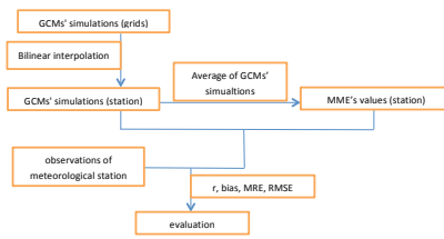
Fig. 1 The flow graph of the accuracy evaluation of GCMs' simulations
