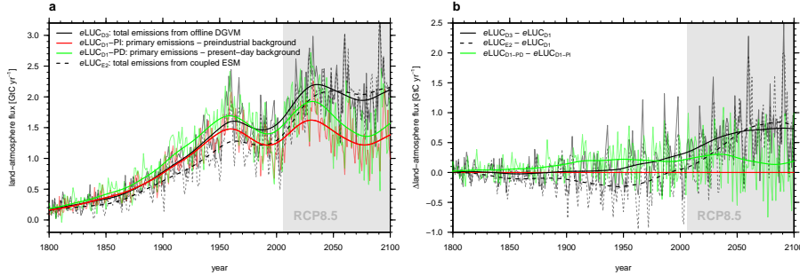
Figure 2. (a) Annual land use change emissions as quantified following different methods. (b) Difference of different eLUC definitions relative to e\text{LUC}_{\text{D1}} , quantified under preindustrial boundary conditions. Total emissions derived from an offline, concentration-driven DGVM setup (D3 method) are given by black solid lines. Total emissions derived from a coupled, emission-driven ESM setup (E2 method) are given by black dashed lines. Primary emissions are given by colored lines under constant pre-industrial (red) and constant present-day (green) environmental conditions (climate, CO 2 , N deposition). Time series are calculated following Eqs. 2-4, where F is the global total land-atmosphere CO 2 flux in the respective simulation. Bold lines are splines of annual emissions given by thin lines. Results are from simulations following CMIP5 model inputs (historical until 2005, RCP8.5 until 2099).
