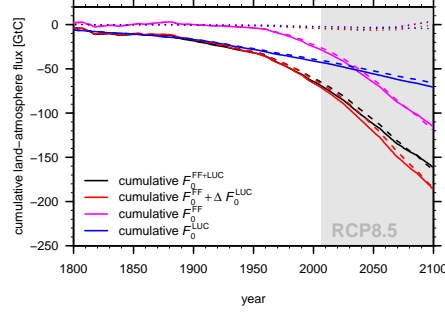
Figure 1. Global cumulative net land-to-atmosphere CO 2 fluxes induced by environmental change caused by FF ( F_0^{\text{FF}} ), LUC ( F_0^{\text{LUC}} ), their combined effect ( F_0^{\text{FF}+\text{LUC}} ), and the sum of individual effects ( F_0^{\text{FF}} + F_0^{\text{LUC}} ). Curves represent cumulative global fluxes induced by environmental change, weighted by their time-varying area of natural vegetation (dashed lines), agricultural land (dotted lines), and their sum (solid lines). Note that this excludes all direct effects of LUC. The difference between the combined and the sum of effects corresponds to the non-linearity (A_0 - \Delta A(t)) \delta_{\text{nat}}(t) + \Delta A(t) \delta_{\text{agr}}(t) . The model setups are described in Tables 1 and 2.
