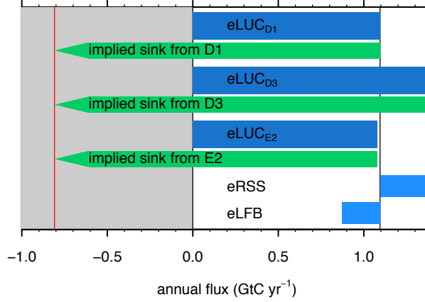
Figure 5. Land use change emissions ( eLUC , dark blue bars) calculated from different methodologies and their implied residual terrestrial C sink (annual flux in GtC\ yr^{-1} , mean over 1996-2005). The total terrestrial C balance is constrained by atmospheric measurements and is -0.8\ GtC\ yr^{-1} (mean over 1996-2005, Le Quéré et al. (2014), left vertical line). It is independent of eLUC estimates. The residual terrestrial C sink (green arrow) is defined as the difference of eLUC and the total terrestrial C balance. Depending on the definition of eLUC , the residual C sink is affected by inclusion of secondary fluxes (light blue bars, eRSS and eLFB ) into eLUC .
