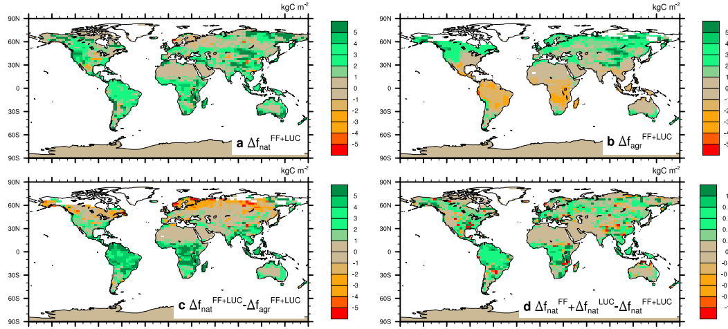
Figure 4. Top row: Cumulative atmosphere-land C flux ( \text{kgC m}^{-2} ) induced by environmental change from 1700 to 2100 on natural (a) and agricultural land (b; mean of cropland and pasture, weighted by respective area shares). The period 2005-2100 follows the RCP8.5 scenario. Climate and \text{CO}_2 are prescribed from the outputs of the coupled simulation (offline simulation F_0^{\text{FF}+\text{LUC}} uses outputs from F_{\text{LUC}}^{\text{FF}+\text{LUC}} ). (c) Difference of flux occurring on natural and agricultural land f_{\text{nat}}^{\text{FF}+\text{LUC}} - f_{\text{agr}}^{\text{FF}+\text{LUC}} . (d) Spatial distribution of non-linear effects, cumulative in year 2100. Its global total over time is expressed also in Figure 1 (difference between black and red curves).
