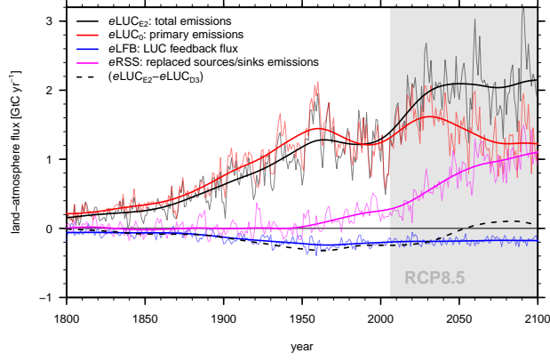
Figure 3. Flux components of land use change emissions. Total emissions as derived from an emission-driven, coupled ESM setup (E2 method), and calculated with Eq. 4, are given by the black lines. Primary emissions under preindustrial boundary conditions are given by red lines. These correspond to curves in Figure 2. The replaced sinks/sources flux ( eRSS ) and the land use change feedback flux ( eLFB ) are given by magenta and blue lines, respectively. The difference between total emissions quantified by D3 method (see black solid line in Fig. 2) and E2 method is given by the black dashed line. Time series are calculated following Eqs. 2, 4, 15, and 16. Bold lines are splines of annual emissions given by thin lines. Results are from simulations following CMIP5 model inputs (historical until 2005, RCP8.5 until 2099).
