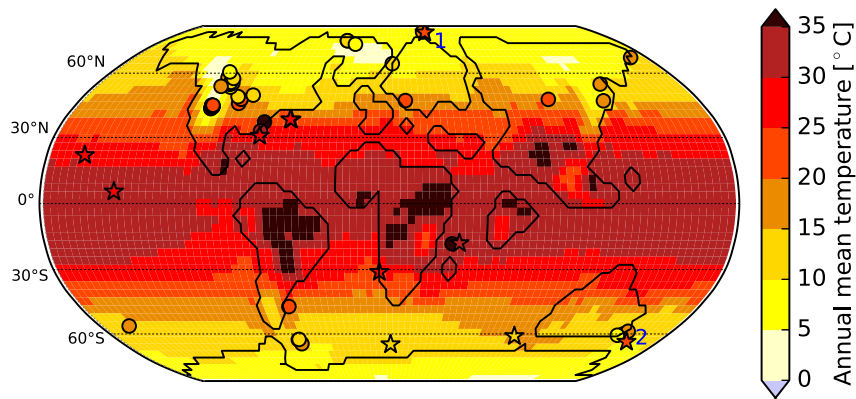
Figure 1. Zonal annual Annual mean 2-m temperature in the initial-early Eocene simulation in comparison to temperature reconstructions shaded colours. Stars show estimates of annual-mean sea-surface reconstructed annual mean sea surface temperature (SST) and near-surface temperature for of the early Eocene based on derived from \delta^{18}\text{O} , Mg/Ca, and TEX 86 (Lunt et al. 2012). Cycles Numbers 1 and 2 mark SST reconstructions by Sluijs et al. (2006) and Bijl (2009), respectively. Circles refer to terrestrial annual mean temperature estimates based on macrofloral and palynoflora assemblage data and from teeth, hydrogen isotopes, and oxygen isotopes (Huber and Caballero 2011).
