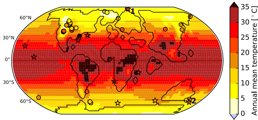
Figure 1. Annual mean 2-m temperature for the early Eocene simulation in shaded colours. Stars show reconstructed annual mean sea surface temperature (SST) and near-surface temperature of the early Eocene derived from \delta^{18}O , Mg/Ca, and TEX 86 (Lunt et al. 2012). Numbers 1 and 2 mark SST reconstructions by Sluijs et al. (2006) and Bijl (2009), respectively. Circles refer to terrestrial annual mean temperature estimates based on macrofloral and palynoflora assemblage data and from teeth, hydrogen isotopes, and oxygen isotopes (Huber and Caballero 2011).
