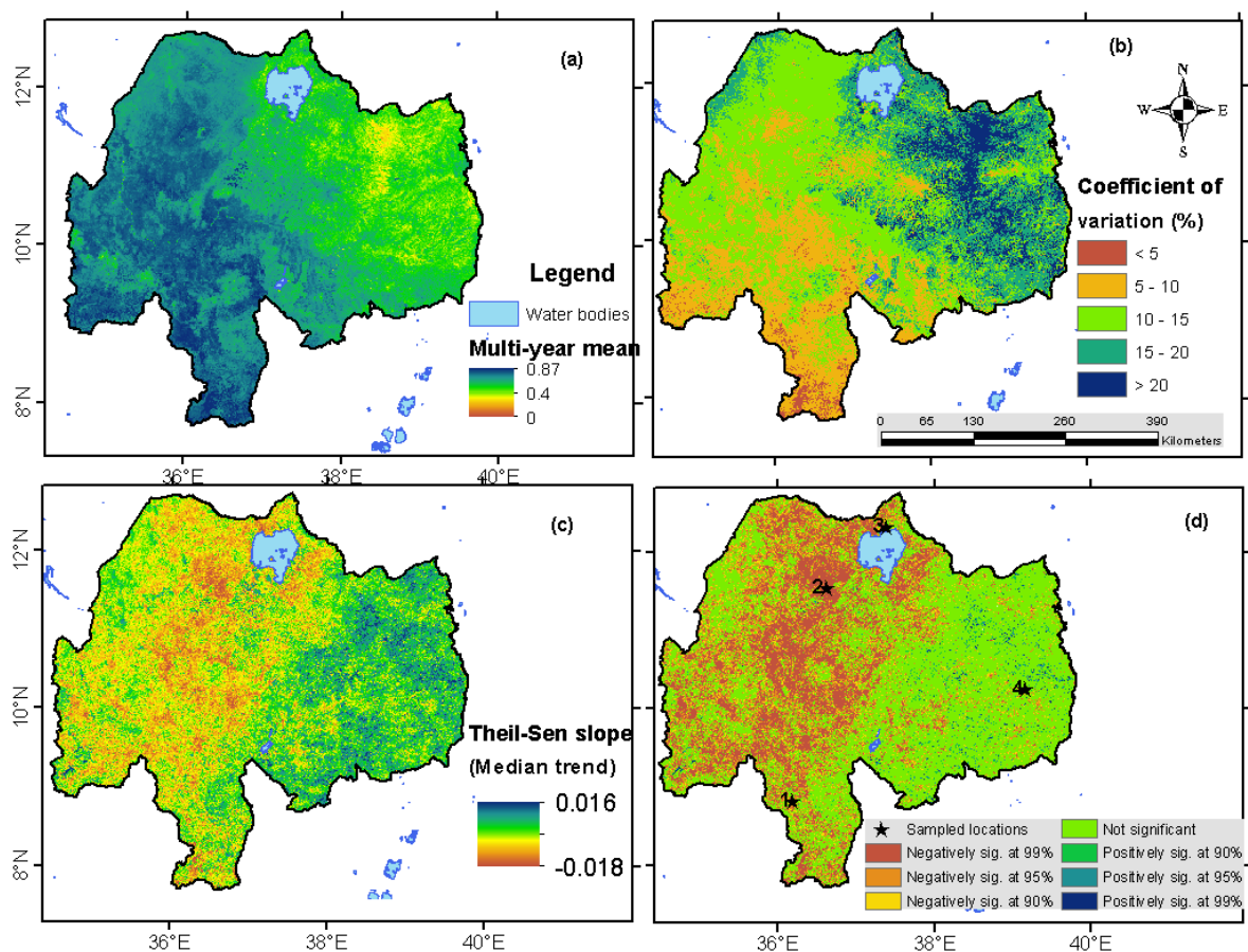
Figure 3. Vegetation cover variability and trends for the Upper Blue Nile (Abay) basin based on MODIS 250m NDVI (MOD13Q1) for the period (2001-2011): (a) multi-year mean monthly NDVI; (b) coefficient of variation of monthly NDVI; (c) Theil-Sen slope ( \Delta\text{NDVI}/\text{month} ); and (d) Mann-Kendall significance test of the trend test.
