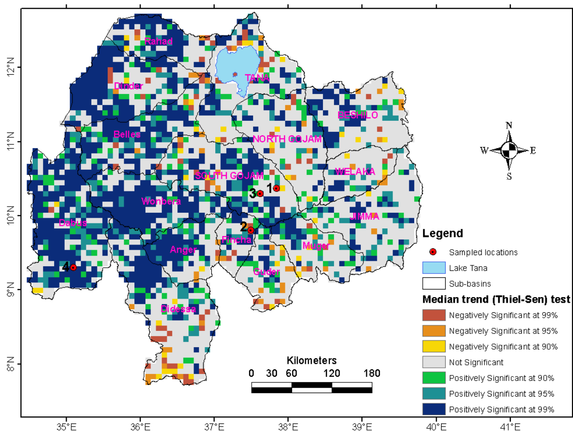
Figure 2. The inter-annual trend in vegetation condition based on GIMMS NDVI in Abay (UBN) basin for the period 1982 to 2006
