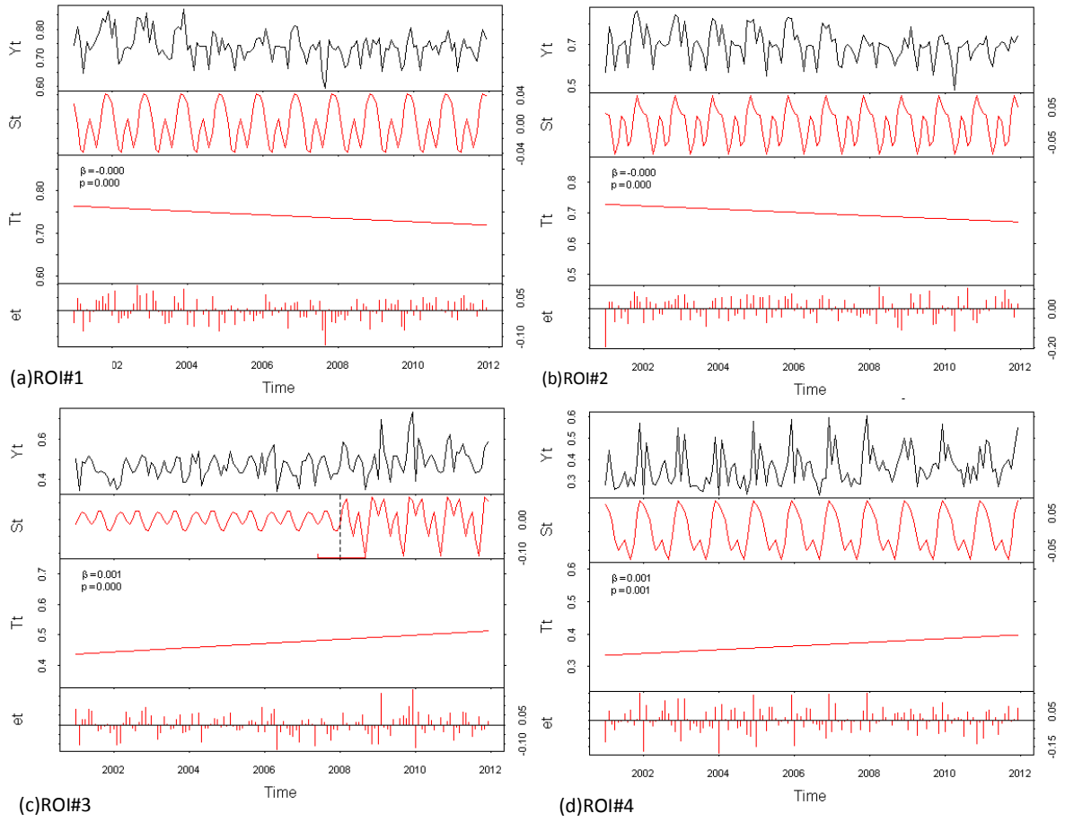
Figure 10. Examples of decomposition and trend break analysis of monthly MODIS NDVI time series (2001-2011) for certain region of interests (ROIs) for significant decreasing trends: (a) ROI #1 and (b) ROI #2 and for significant increasing trends: (c) ROI #3 and (d) ROI #4 generated by BFAST approach. The locations of ROIs are shown in Fig. 3 (d). The top panel in every plot shows the NDVI data, whereas the other three panels depict the individual components after decomposition. The seasonal ( S_t ) and remainder ( e_t ) components have zero mean while the trend component ( T_t ) shows the trend in NDVI. The slope coefficients ( \beta ) and the significance levels ( P ) at \alpha value of 0.05 for each segment are given.
