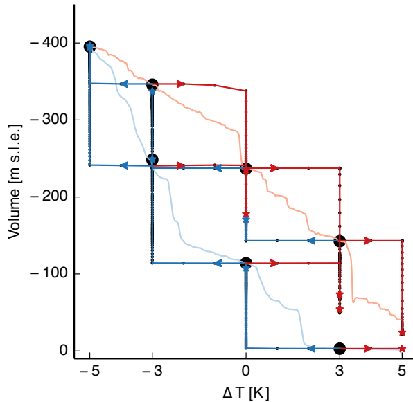
Figure 13. Global ice volume of simulations with a rapid temperature transitions of 1\text{ }^{\circ}\text{C}/1000\text{ years} . Base of the transition simulations is the hysteresis simulation from figure 11 (b) which is shown as pale background. The large black dots are identical to the dots in figure 11 and mark the equilibrium state at the specific temperature. Simulations are started from \{-3, 0, +3\}\text{ }^{\circ}\text{C} with temperature increase (red) or decrease (blue) of 1\text{ }^{\circ}\text{C}/1000\text{ years} and a runtime of 100,000 years (small black dots every 1000 years) until equilibrium (asterisks). The temperature difference of 3\text{ }^{\circ}\text{C} is constantly applied in the first 3000 years and held stable after then.
