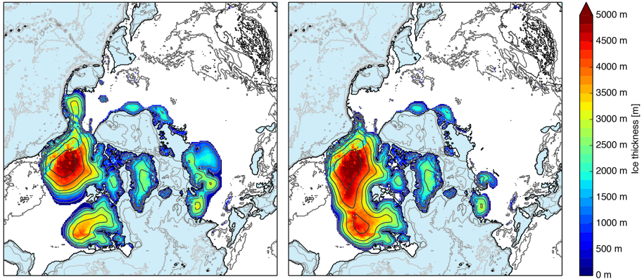
Figure 8. Ensemble composite of all simulations within LGM ice volume range of -132 and -95 m.s.l.e. (see gray horizontal bar in Fig. 7) (Clark and Mix, 2002). Ensemble LGM_{uc} (left, mean -111.9 m.s.l.e. ) consists of 50 simulations, and LGM_{bs} climate forcing (right, mean -114.7 m.s.l.e. ) has 114 members.
