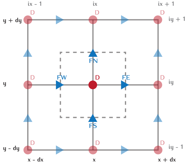
Figure 1. Schematic representation of the model grid. Ice thickness h , bedrock elevation b and diffusivity D are calculated on regular grid points (ix, iy) . Halfway between these points, the lateral flux (FN, FS, FW, FE) of ice is calculated on staggered grid points.
