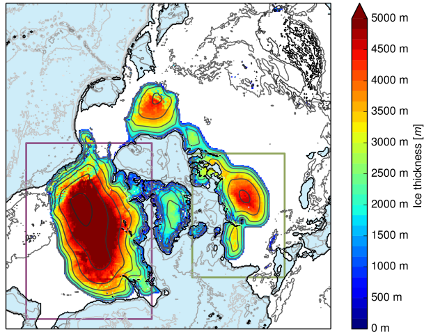
Figure 12. Hysteresis after 3.75 mio years at LGM temperature ( \Delta 0^\circ\text{C} ) with an ice volume of 236.7 m SLE. The situation at the same temperature at the build up process of the ice sheet after 1.25 mio years can be seen in Fig.9 (left). Areas of North America and Eurasia from Fig. 11c and d are enclosed in purple and green boxes, respectively.
