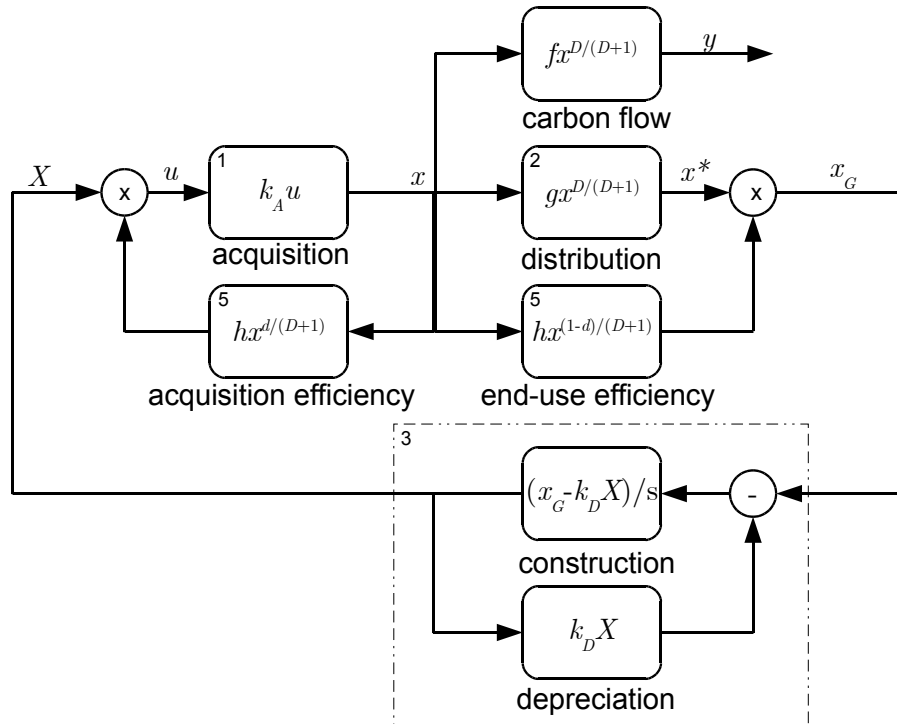
Figure 5. The system diagram representation of the endogenous growth model set out in Eqs. (1)–(5). Numbers in boxes denote which equations apply. s in the “construction” transfer function is the derivative operator, d/dt .
