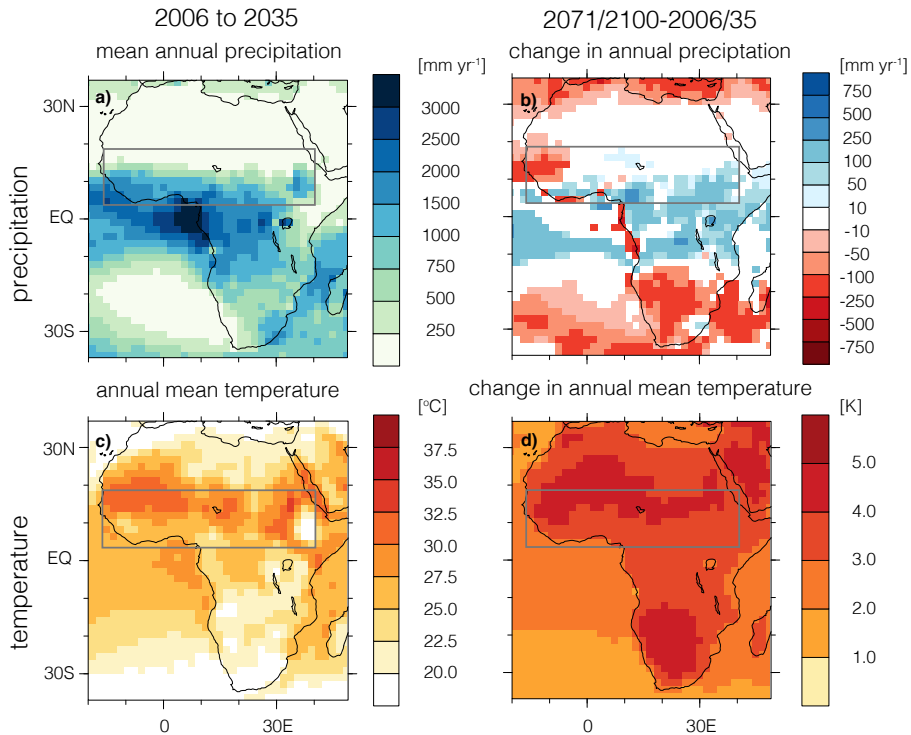
Figure 3. (a, c) Ensemble mean annual precipitation sum [mm] and temperature [°C] for the first 30 years of RCP8.5 scenario (2006 to 2035) (left column) and (b, d) the difference (right column) with respect to the last 30 years of this century (2071 to 2100 minus 2006 to 2035). Only significant differences ( t test, 95% significance level) are show. Both, small changes in precipitation and non significant changes are in white colour (b).
