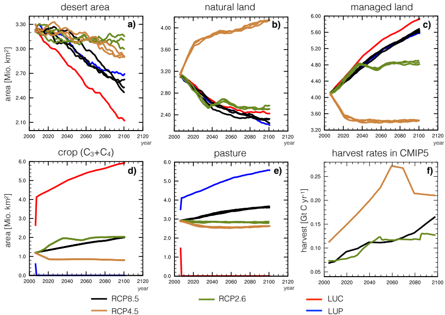
Figure 4. Top row: temporal course of the simulated desert area (a), natural (b), and managed (c) land within three different CMIP5 scenarios and two land use scenarios (LUC,LUP) within the next century (2006 to 2100). Bottom row: changes of anthropogenic land use within the next century is given for crops (d) and pasture (e) separately. Values are given in Mio. km 2 . The different harvest rates within the CMIP5 scenarios are shown in (f). Shown are integrated values only for our area of interest, where the strong land use experiments take place. The dashed and dotted black lines represent the three ensemble member of the RCP8.5 scenario, while the dashed one marks the ensemble member based on the same restart (year 2005) as the land use experiments for this study.
