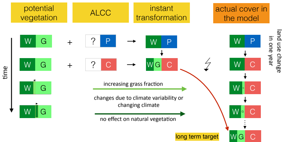
Figure A1. Diagram to illustrate the legacy effect of long term changes in natural vegetation (G: grass, W: woody type) after strong anthropogenic land use transitions (P: pasture, C: crop). Shown are the potential vegetation (model internal) which is in equilibrium with the current climate, the prescribed transition, the instant transformation of the left two informations into a grid cell, and the actual, simulated cover (right column), which accounts for slow changes in-between two successive years within the natural vegetation.
