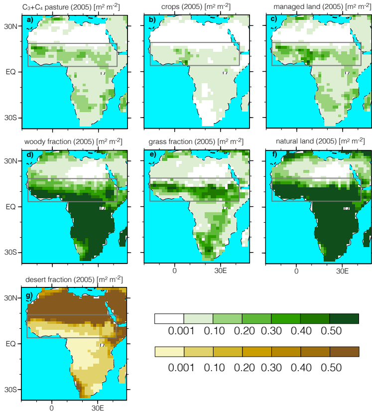
Figure 2. Ensemble mean of the cover fraction [ m^2 m^{-2} ] of managed land (top), natural vegetation (middle), and desert fraction (bottom) at the end of the historical simulation (year 2005) simulated by MPI-ESM. The managed land is shown for (a) pasture, (b) crops, and (c) total fraction. The natural vegetation is shown for (d) woody vegetation, (e) grass land, and (f) total separately.
