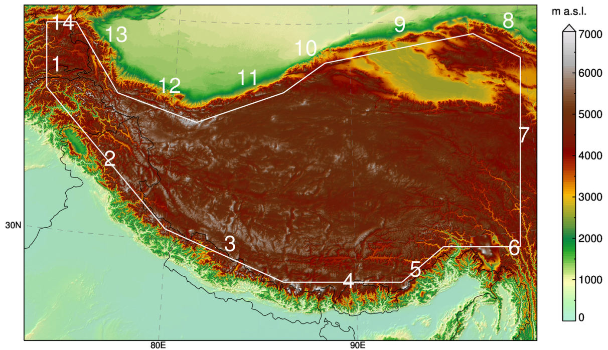
Figure 1: Map of HAR10 domain with cross sections (1-14) slightly moved towards the center of the TP (compare Fig. 1 in the manuscript).
