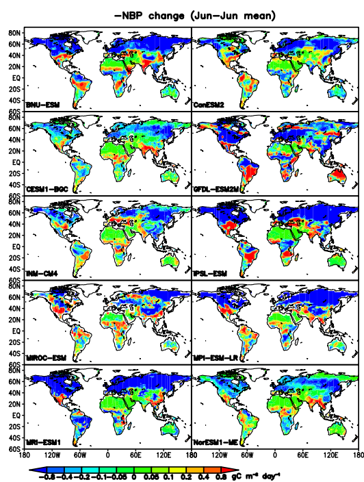
Fig. 2. Spatial patterns of -NBP changes in June for the 10 models.
