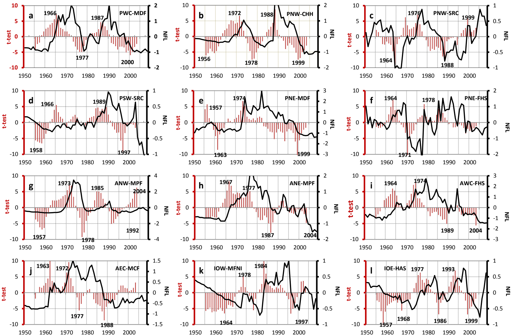
Figure 3 , The detrended time series of selected normalized fish landings shown with black curves over the three ocean basins (scaled by right Y-axis), and the 11-year running t-test with red bars (scaled by left Y-axis). The number indicates the year when the regime shift occurred, based on passing the significance test at the 90% confidence level. Each panel in this figure is a sample selected from the 126 total plots (14 sub-regions and 9 species group combinations) listed in Table A1. Shown are: Pacific Ocean : (a) PWC-MDF; (b) PNW-CHH; (c) PNW-SRC, (d) PSW-SRC ; (e) PNE-MDF; (f) PNE-FHS; Atlantic Ocean : (g) ANW-MPF; (h) ANE-MPF; (i) AWC-FHS; (j) AEC-MCF; Indian Ocean : (k) IOW-MFNI; (l) IOE-HAS. All regime shift years derived from this analysis are listed in Table 2A from the 126 plots.
