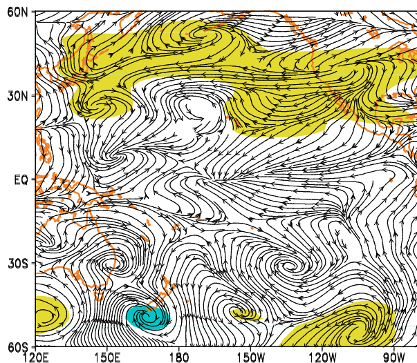
Fig.8 Pacific Ocean reconstructed height (shaded) and wind field anomalies (streamlines) over the Pacific ocean at the 1000hPa model level (surface) for planetary wave numbers 1 thru 6. Shaded areas indicate the height anomalies exceeding the significance test at the 95% confidence level. (Negative anomaly : Blue-purple shading; Positive anomaly : Green-yellow-red). Period: (a) 1948-56; (b) 1957-64; (c) 1965-77; (d) 1978-88, (e) 1989-98, (f) 1999-2005. Coastline in orange. Note, the domain shown is from 60°S to 60°N to highlight regions of wind driven forcing over the Pacific Ocean. When the streamlines converge, the water is generally rising or sinking (upwelling and downwelling).
