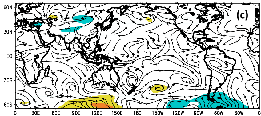
Fig.7 Global regime shift period reconstructed height (shaded) and wind field anomalies (streamlines) at 1000hPa model level (surface) for planetary wave numbers 1 thru 6. Shaded areas indicate height anomalies exceed the significance test at the 95% confidence level. (Negative anomaly : Blue-purple shading; Positive anomaly : Green-yellow-red). Period: (a) 1948-56; (b) 1957-64; (c) 1965-77; (d) 1978-88, (e) 1989-98, (f) 1999-2005. Note, the domain shown is from 60°S to 60°N.
