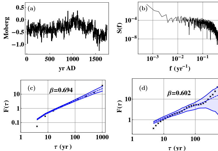
Fig. 2. (a) The Moberg reconstructed temperature. (b) PSD, (c) DFA2 and (d) WVA2 applied to the record. The blue areas are the 95 % confidence for synthetic fGn with \beta estimated with DFA2 and WVA2, indicated in the figure.
