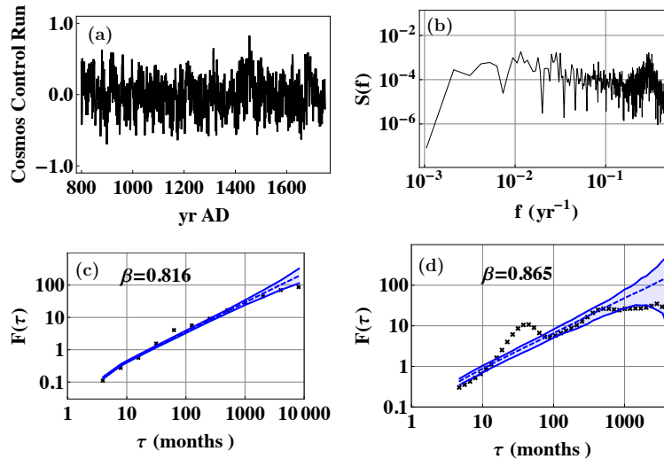
Fig. 7. (a) The temperature from the COSMOS controlrun. (b) PSD, (c) DFA2 and (d) WVA2 applied to the record. The blue areas are the 95 % confidence for synthetic fGn with \beta estimated with DFA2 and WVA2, indicated in the figure.
