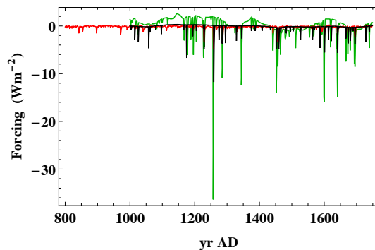
Fig. 1. The different forcings used as input to the response model, i.e. Crowley forcing used with the Moberg reconstruction (black), forcing used in the COSMOS experiment (red) and forcing used in the LOVECLIM experiment (green).
