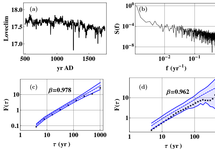
Fig. 4. (a) The temperature from the LOVECLIM experiment. (b) PSD, (c) DFA2 and (d) WVA2 applied to the record. The blue areas are the 95 % confidence for synthetic fGn with \beta estimated with DFA2 and WVA2, indicated in the figure.
