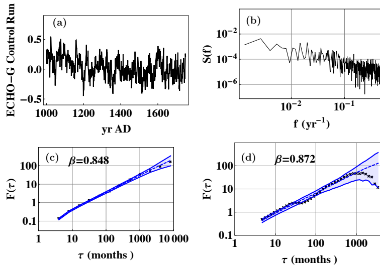
Fig. 10. (a) The temperature from the ECHO-G controlrun. (b) PSD, (c) DFA2 and (d) WVA2 applied to the record. The blue areas are the 95 % confidence for synthetic fGn with \beta estimated with DFA2 and WVA2, indicated in the figure.
