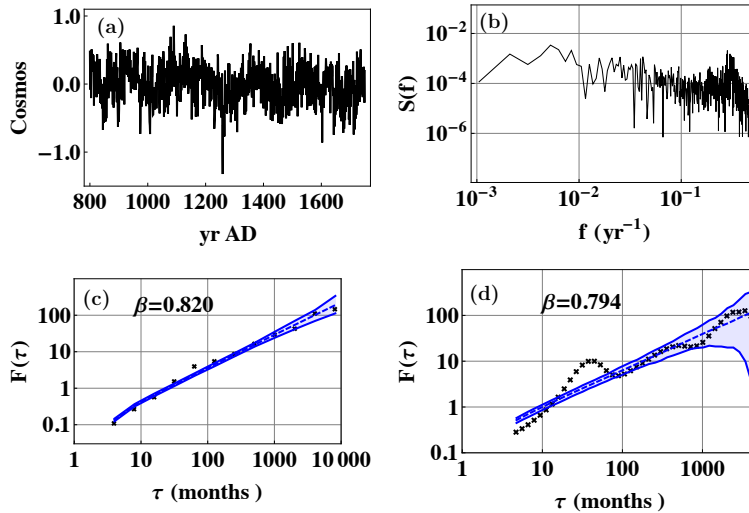
Fig. 6. (a) The temperature from the COSMOS experiment. (b) PSD, (c) DFA2 and (d) WVA2 applied to the record. The blue areas are the 95 % confidence for synthetic fGn with \beta estimated with DFA2 and WVA2, indicated in the figure.
