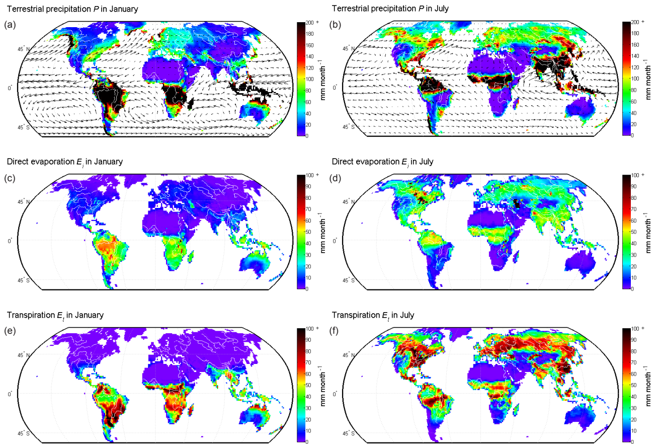
Fig. A2. Precipitation and evaporative fluxes for January (left column) and July (right column).
