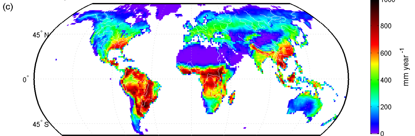
Fig. A1. Average continental precipitation and evaporative fluxes (1999–2008). (a) Precipitation (b) Direct evaporative flux, dominated by interception (Eq. 2), and (c) Delayed evaporative flux, i.e., transpiration (Eq. 3). The arrows in (a) indicate the vertically integrated moisture fluxes.
