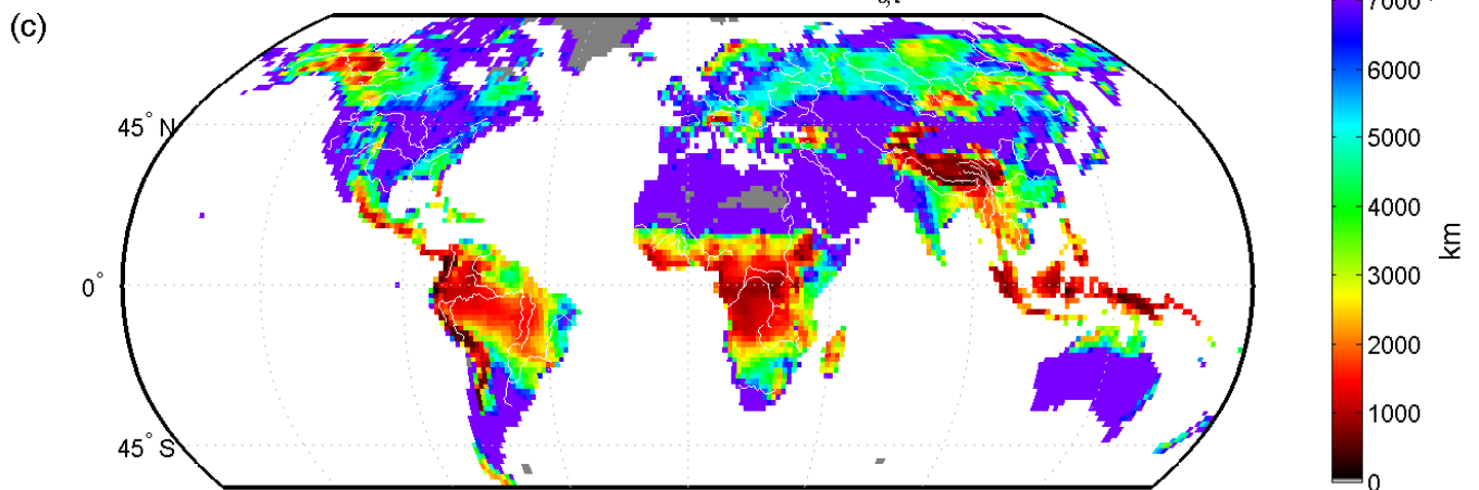
Fig. 5. Local length scales of the moisture recycling process (1999–2008). (a) length scale of precipitation recycling \lambda_\rho , (b) length scale of evaporation recycling for interception \lambda_{\varepsilon,i} , and (c) length scale of evaporation recycling for transpiration \lambda_{\varepsilon,t} . Grey values on land indicate no data, due to the fact that the evaporative flux in question is zero. Note that lower values indicate higher moisture feedback strength. The arrows in (a) indicate the moisture fluxes in the lowest part of the atmosphere (approximately the lowest 2 km of the atmosphere at standard pressure, Eq. (B5)).
