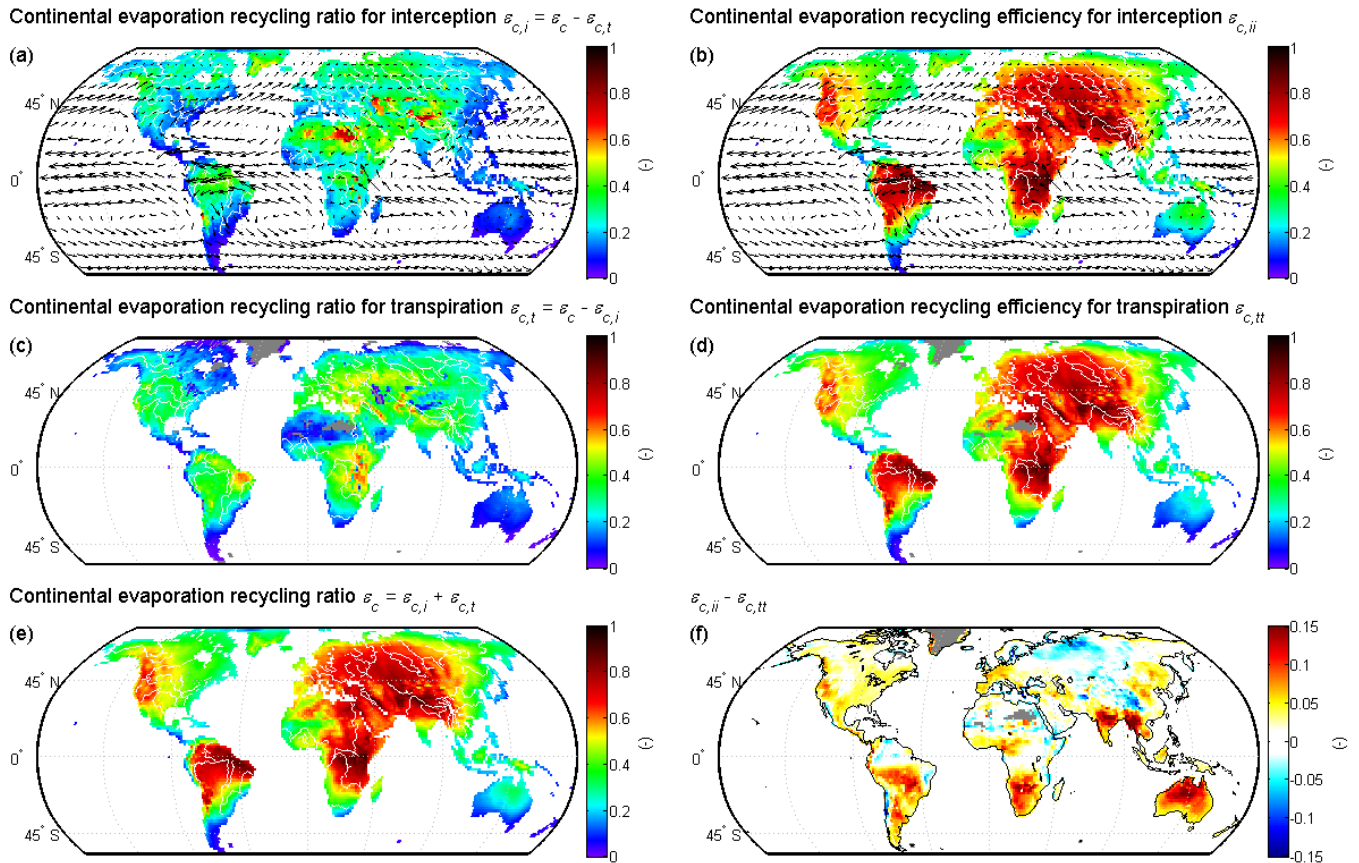
Fig. 3. Continental evaporation recycling (1999–2008). (a) continental evaporation recycling ratio for interception \varepsilon_{c,i} , (b) continental evaporation recycling efficiency for interception \varepsilon_{c,ii} , (c) continental evaporation recycling ratio for transpiration \varepsilon_{c,t} , (d) continental evaporation recycling efficiency for transpiration \varepsilon_{c,tt} , (e) continental evaporation recycling ratio \varepsilon_c , and (f) \varepsilon_{c,ii} - \varepsilon_{c,tt} . Grey values on land indicate no data, due to the fact that the evaporative flux in question is zero. The arrows in (a) and (b) indicate the vertically integrated moisture fluxes.
