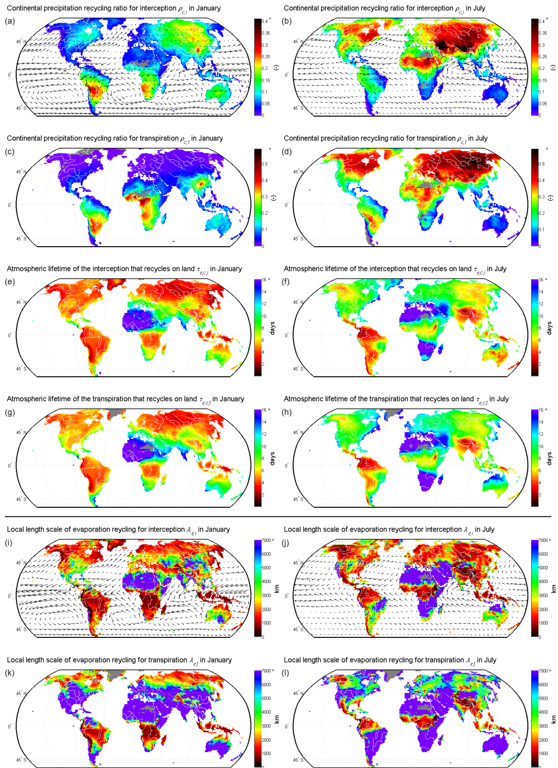
Fig. 6. Moisture recycling metrics for January (left column) and July (right column). The arrows in (a) and (b) indicate the vertically integrated moisture fluxes, which are most relevant for panels (a–h). The arrows in (i) and (j) indicate the moisture flux only in approximately the lowest 2 km of the atmosphere, which is most relevant for panels (i–l).
