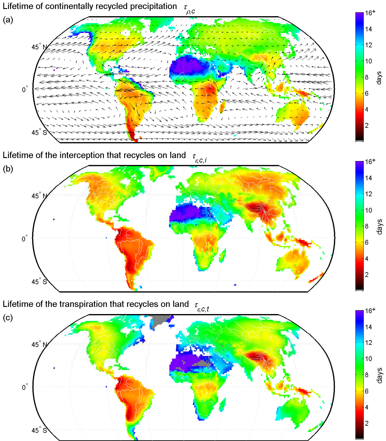
Fig. 4. Average atmospheric lifetimes of recycled moisture (1999–2008). (a) lifetime of continentally recycled precipitation \tau_{\rho,c} (defined at the point of precipitation), (b) lifetime of the interception that recycles on land \tau_{\varepsilon,c,i} (defined at the point of evaporation), and (c) lifetime of the transpiration that recycles on land \tau_{\varepsilon,c,t} (defined at the point of evaporation). Grey values on land indicate no data, due to the fact that the evaporative flux in question is zero. The arrows in (a) indicate the vertically integrated moisture fluxes.
