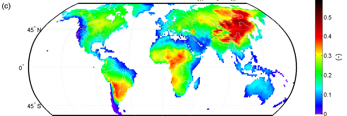
Fig. 2. Continental precipitation recycling (1999–2008). (a) continental precipitation recycling ratio \rho_c , (b) continental precipitation recycling ratio for interception \rho_{c,i} , and (c) continental precipitation recycling ratio for transpiration \rho_{c,t} . The colour scale of (b) ends at 0.41, which is the global average fraction of direct evaporative fluxes (interception) and the colour scale of (c) ends at 0.59, which is the global average fraction of delayed evaporative flux (transpiration). The arrows in (a) indicate the vertically integrated moisture fluxes.
