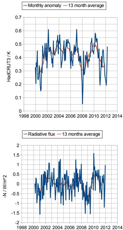
Fig. 1. Comparison of monthly anomalies and 13 months averages. Temperature (top), Net radiative flux (bottom).
