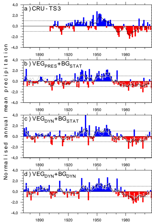
Fig. 3. Annual mean precipitation normalised w.r.t. mean and the standard deviation of rainfall for the years 1901–2006 in the Sahel. (a) Observed precipitation from the CRU-TS3 land data set (Mitchell and Jones, 2005), bars show yearly values, lines show five-year running averages. Simulated precipitation for the (b) static ( VEG_{PRES} + BG_{STAT} ) simulations, (c) dynamic vegetation ( VEG_{DYN} + BG_{STAT} ) simulations, (d) dynamic vegetation and dynamic albedo ( VEG_{DYN} + BG_{DYN} ) simulations. Bars show annual values of the ensemble mean. Lines show five-year running averages for the individual ensemble members (grey) and the ensemble mean (black). The dotted lines indicate one standard deviation from the mean.
