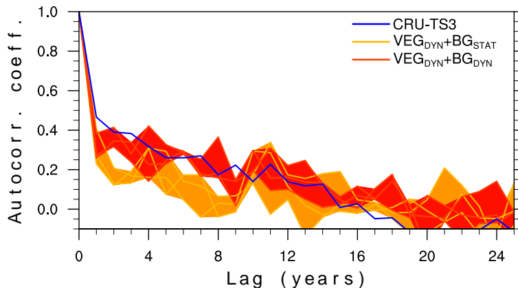
Fig. 5. Autocorrelation function calculated for the years 1901–2006 for observed precipitation (CRU–TS3) and for simulated precipitation of the ensemble members for VEG DYN +BG STAT and VEG DYN +BG DYN simulations. Shadings indicate the ensemble spread.
