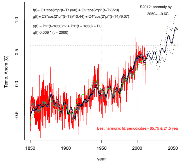
Fig. 2. A reproduction of Fig. 5 in Scafetta, 2012a (also available on-line from http://arxiv.org/pdf/1201.1301v1.pdf ). The reproduction was done calling the function “Scafetta2012( )” in replicationDemos. The grey horizontal dashed line marks the level where Scafetta’s curve intersects year 2050. An interactive search for periodicities in the vicinity of those suggested by Scafetta, gave a best fit to the pair of harmonics if they were 21.5 and 65.75 yr respectively.
