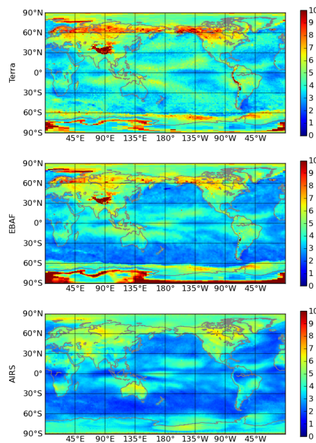
Fig. 2. Standard deviation of the anomaly time series at each grid point. In W/m^2 .
